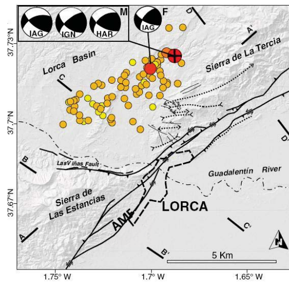
Figure 1. Map of relocated instrumental epicenters of the Lorca sequence until July 7 2011, with the focal mechanism of the foreshock and the mainshock. AMF: Alhama de Murcia fault. (Modified from Martínez-Díaz et al. 2012 and López-Comino et al. 2012).
