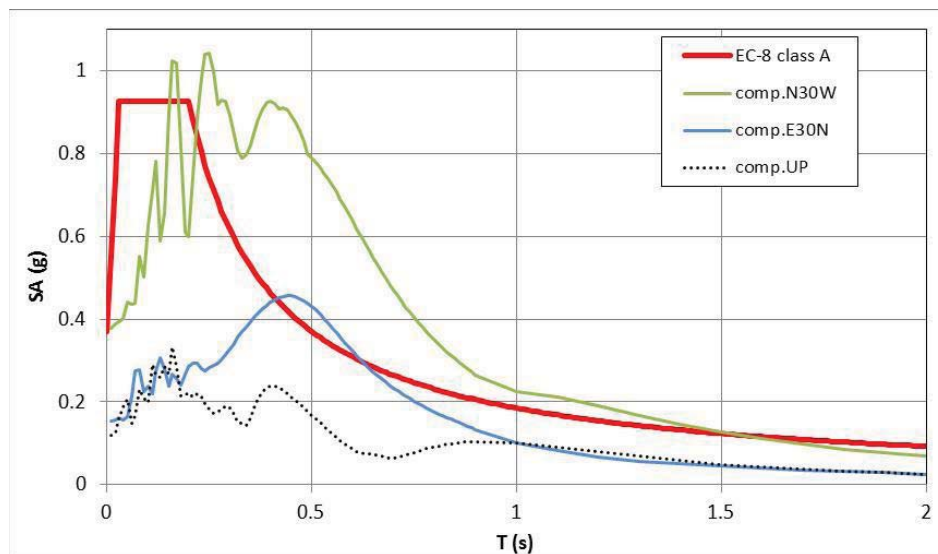
Figure 6. Comparison of EC8 Type 2 acceleration response spectra scaled to PGA of 0.37 g with the spectra from the recorded horizontal ground motion at the LOR station (5 km from the source).
