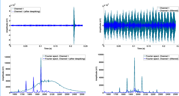
Time-serie and spectrum before/after despiking (left) and before/after sinusoidal subtraction (right): the channel 1 signal is made of a synthetic signal embedded in real noise measurements. The synthetic signal takes the form: MRS(t) = E_0 \cos(2\pi f_0 t + \phi) \cdot \exp(-t/T_2) .
