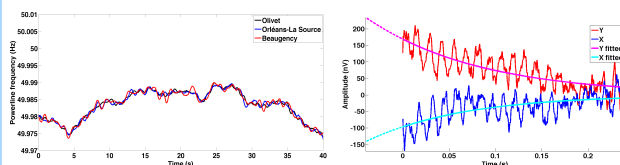
Fundamental powerline frequency synchronously measured in three locations (at the regional scale: ~30km distance).
