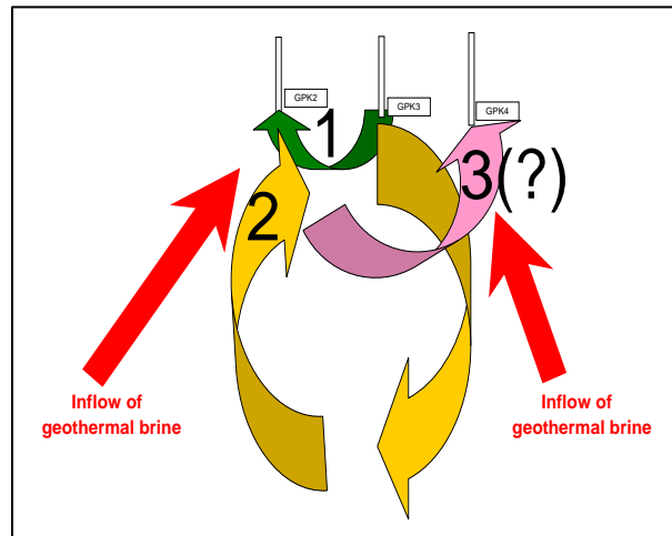
Figure 2: Conceptual model of fluid circulation in the Soultz EGS site: 1. Short scale loop between GPK-3 and GPK-2; 2. Large scale loop between GPK-3 and GPK-2; 3. Connection between the large scale loop and GPK-4 (from Sanjuan et al. , 2006a).
