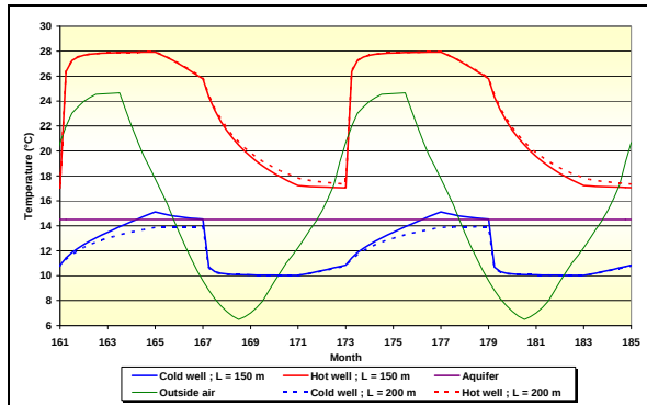
Figure 10: Comparison of the simulated temperatures in the cold and hot wells for L = 150\text{m} and 200\text{m} , i = 0.4\% ; Q = 50 \text{ m}^3/\text{h} , Aquifer thickness = 10\text{m} , Cover thickness = 20\text{m} , K = 5.10^{-3} \text{ m/s} , \varepsilon = 15\% .
