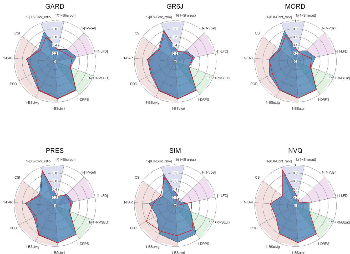
Figure 9. Radial plot of the mean model results for the 21 catchments for the selected criteria in validation period 2, for a d + 30 forecasting lead time. Red lines represent the results when no assimilation or post correction method is used.
