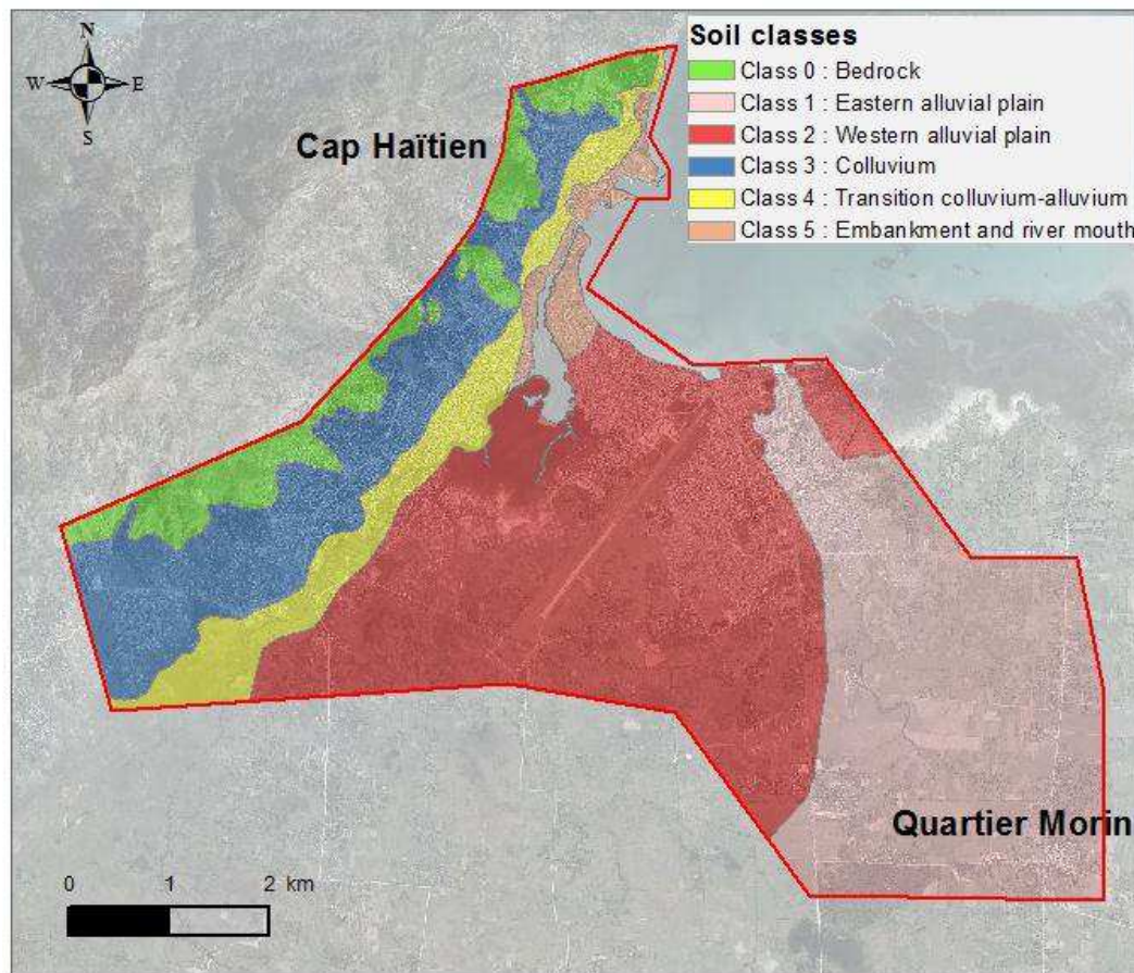
Figure 8. Soil classes zoning for Cap Haitien area. Class 0 represents bedrock at the outcrop surface.
