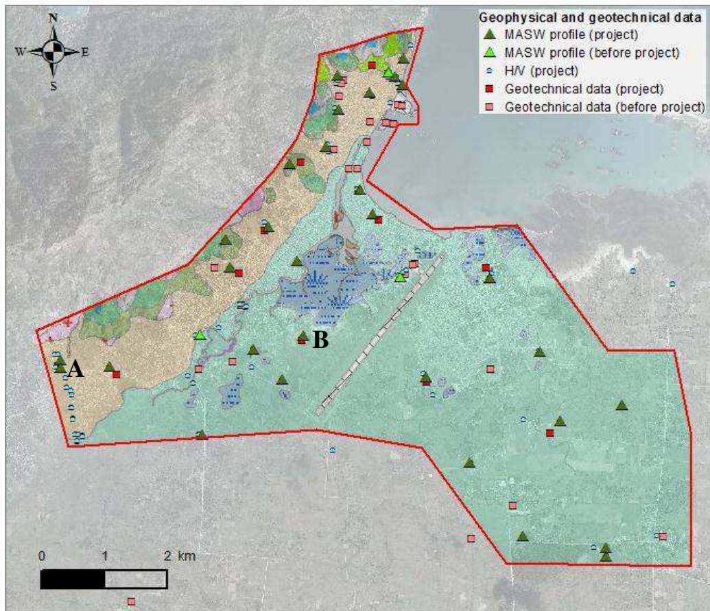
Figure 3. Main data used for site effect zoning. See the legend of Figure 2 for geological background. H/V spectral ratios, MASW and SPT profiles for the sites A (cité administrative) and B (centre éducatif Suzanne Flon) are illustrated on Figure 5 and Figure 6.
