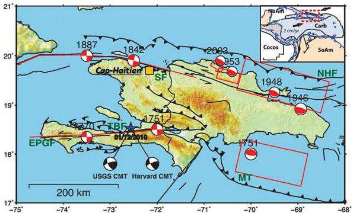
Figure 1. Seismotectonic setting of Hispaniola from Douilly et al. (2013). The January 2010 earthquake is shown with a blue star and black focal mechanisms. Cap-Haitien is displayed as a yellow square. The city is on the vicinity of the Septentrional Fault (red line named SF) and has been totally destroyed by the M8 earthquake of 1842. Other main historical earthquakes are shown (years in black and red focal mechanisms)
