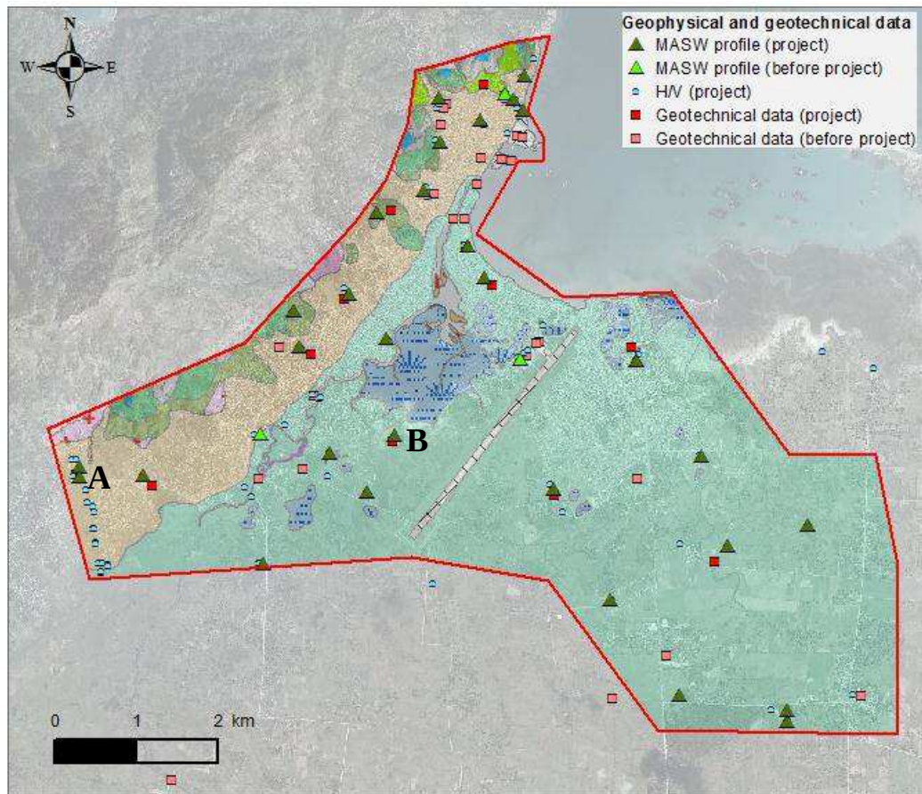
Figure 3. Main data used for site effect zoning. See the legend of Figure 2 for geological background. H/V spectral ratios, MASW and SPT profiles for the sites A (cit  administrative) and B (centre  ducatif Suzanne Flon) are illustrated on Figure 5 and Figure 6.
