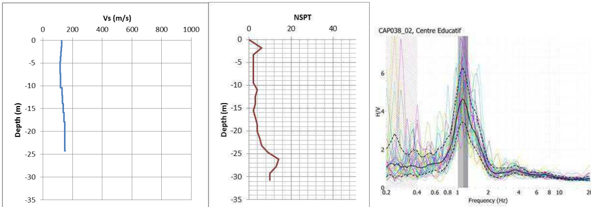
Figure 6. MASW profile, SPT profile and H/V curves for Point B.
