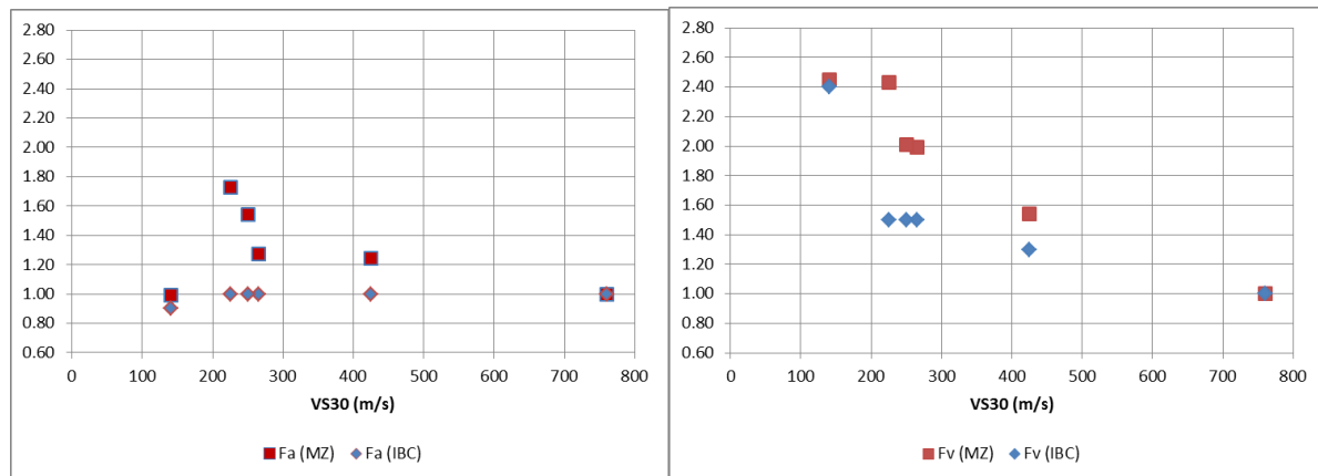
Figure 10. Comparisons of amplification factors Fa (left) and Fv (right) found for this microzoning (MZ) and proposed in IBC code.
