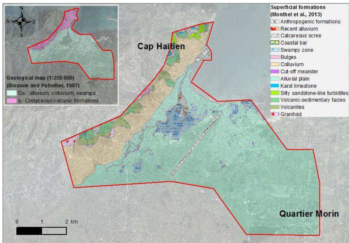
Figure 2. Geological map reassessed for the project at a 1: 25 000 scale. On top left, the geological map at 1:250 000 from Boisson & Pubellier (1987). The studied area is represented by the red line.
