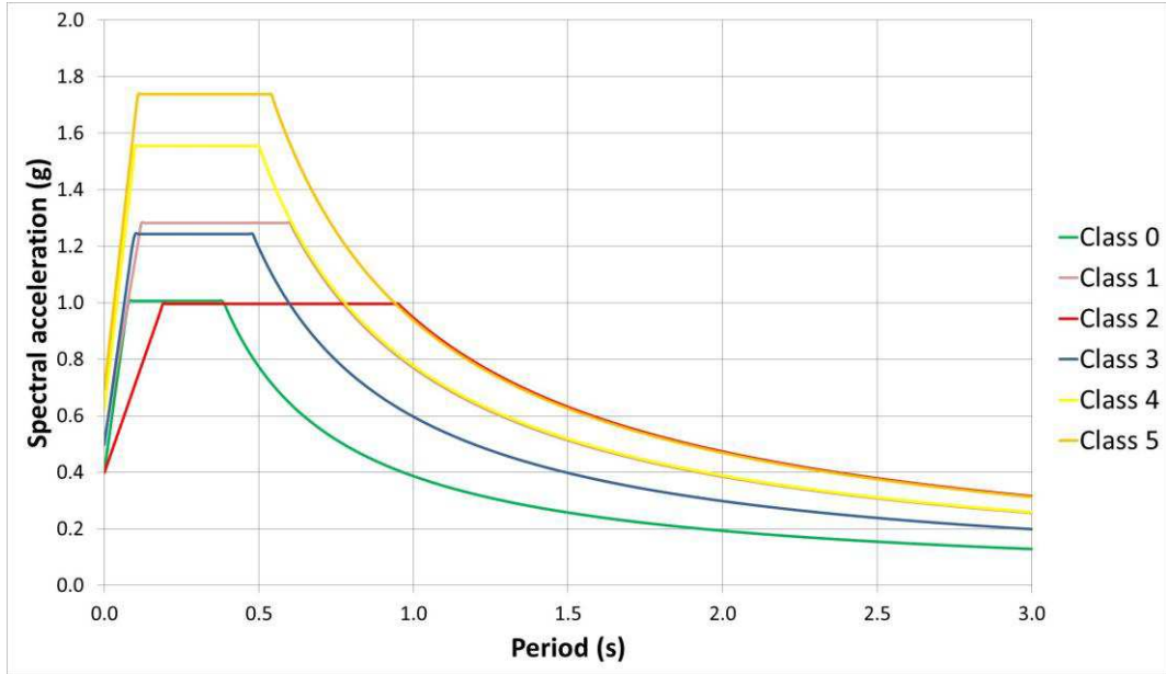
Figure 9. Elastic response spectra for the 6 soil classes. Spectrum for outcropping bedrock (Class 0) is represented in green.
