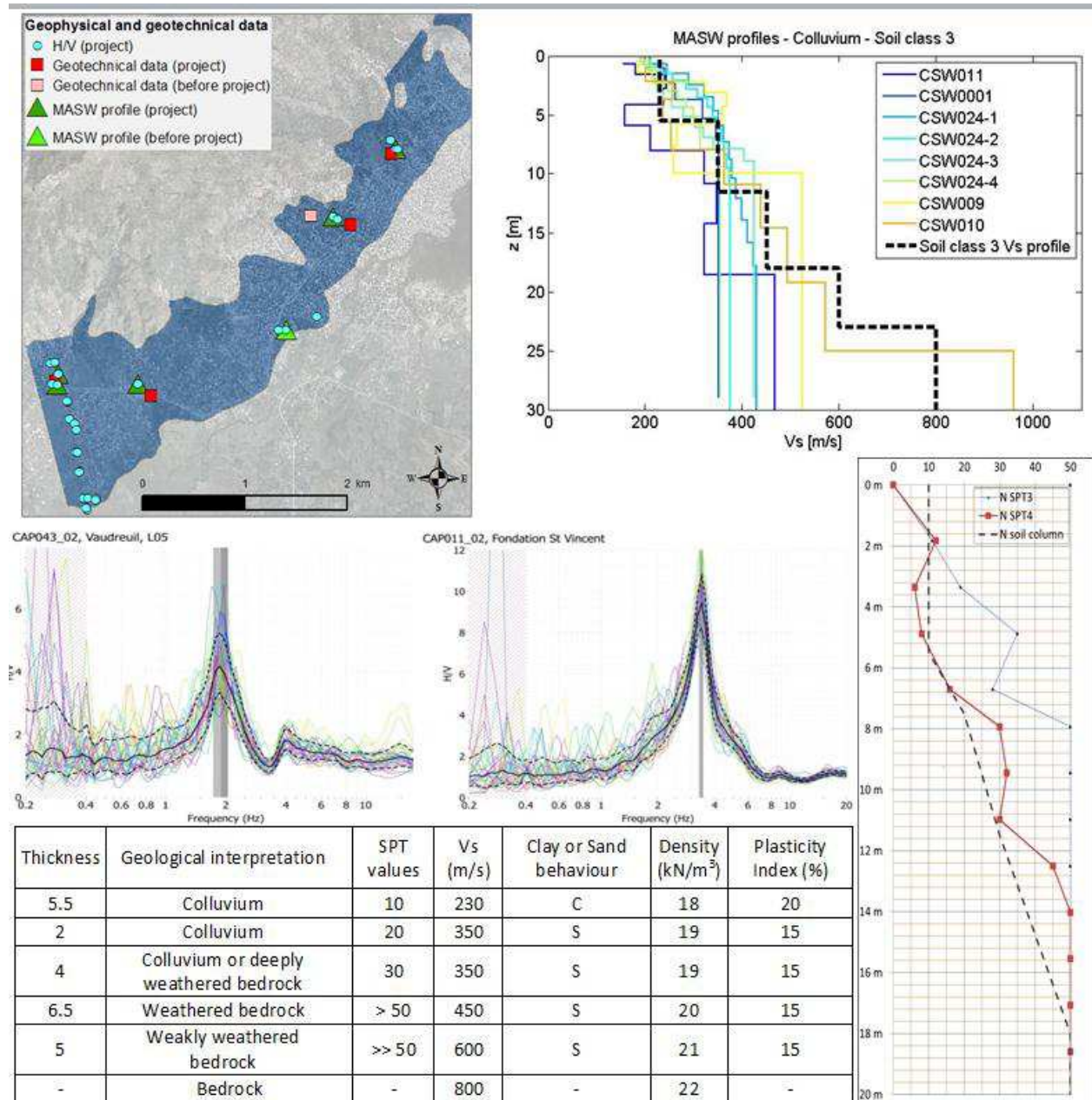
Figure 7. Column of soil for the colluvium area (part of class 3 of the final microzoning) and examples of H/V peaks, MASW profiles and NSPT profiles.
