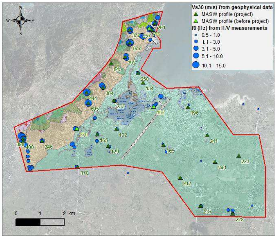
Figure 4. Joint interpretations of geological and geophysical measurements.
