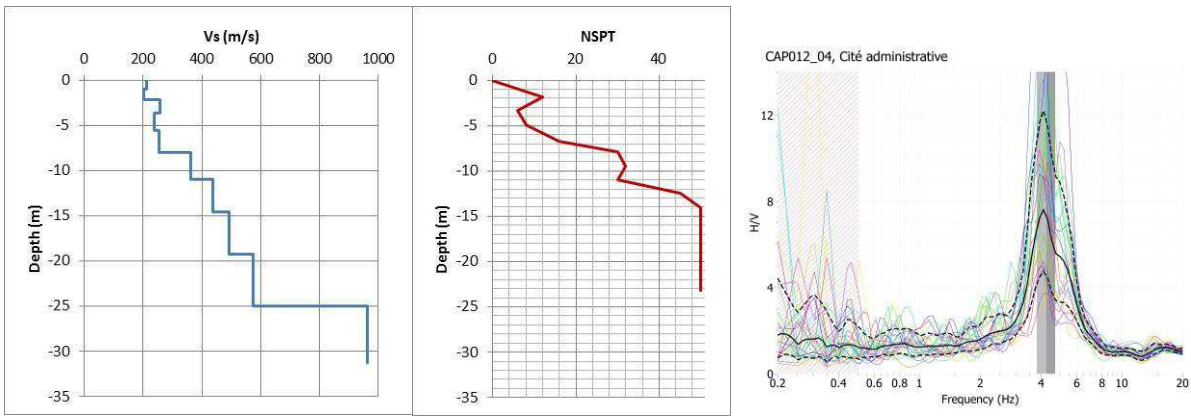
Figure 5. MASW profile, SPT profile and H/V curves for Point A
