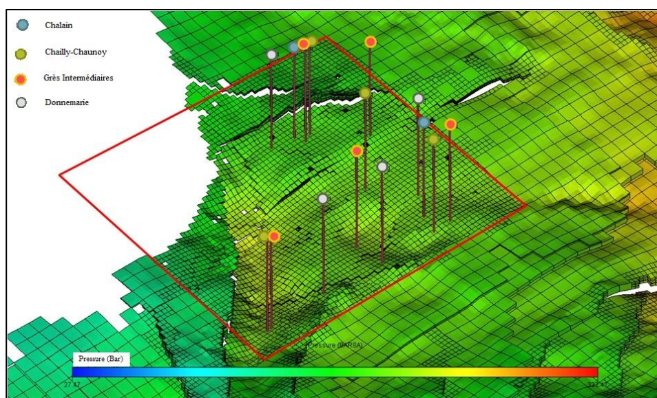
Fig. 4- "Keuper Sud" model with grid refinement around the injection zone and along the faults. The 15 wells necessary to inject from 54 to 140 Mt are represented with their stratigraphic target.
