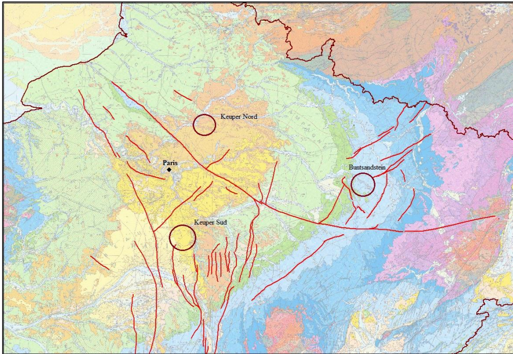
Fig. 3 – Study area in the northern part of France with the common structural pattern chosen for the project (red lines). The 3 sites selected at the end of the regional modeling are represented by circles.
