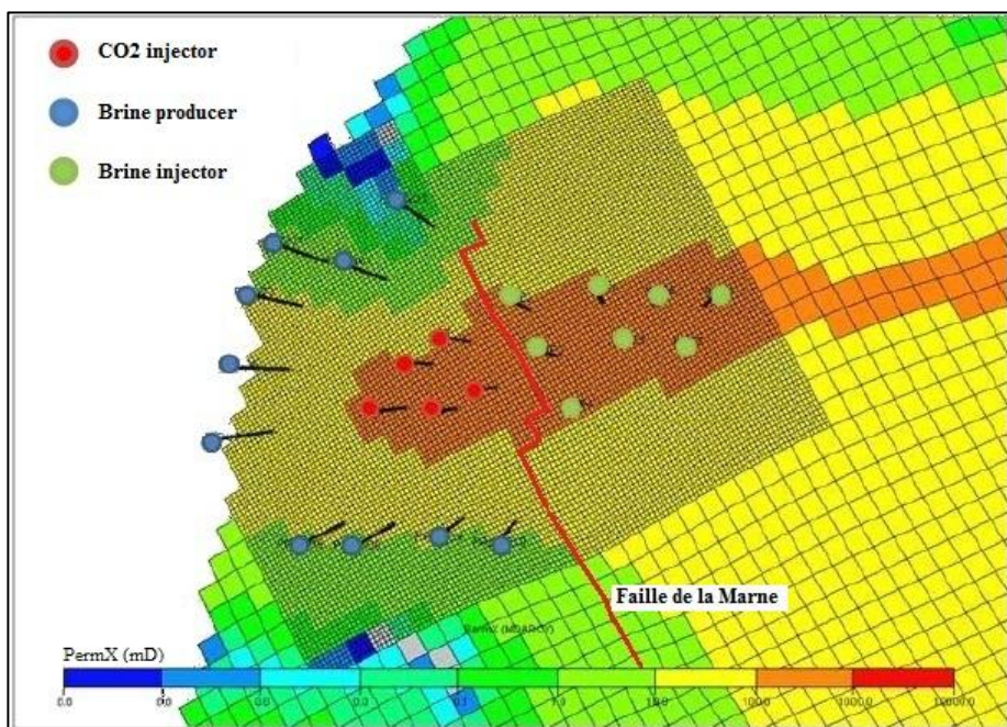
Fig. 5- Site model of Buntsandstein site with grid refinement. Wells configuration as for the injection west of the Marne Fault (“Faille de la Marne” represented by the red line).
