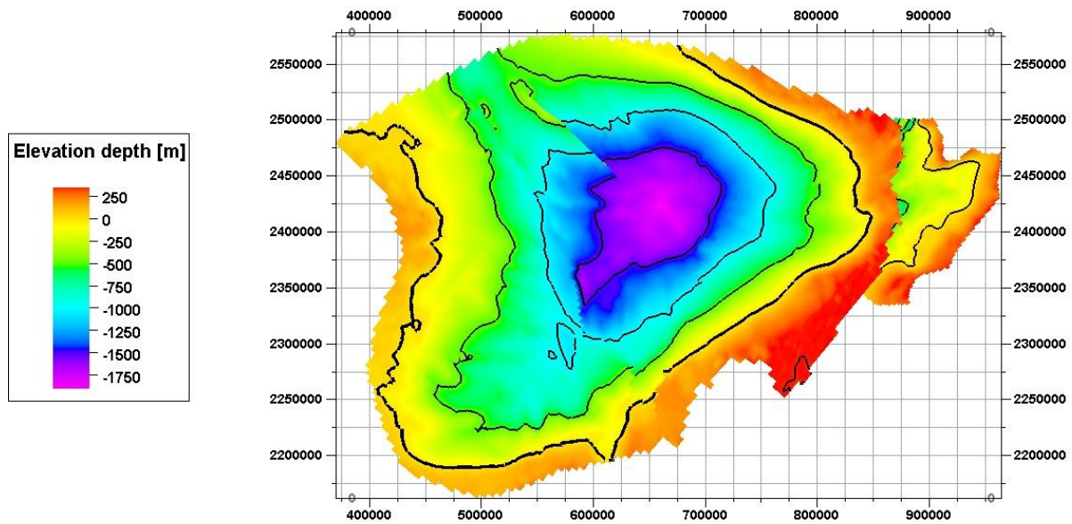
Fig. 2- Map view of the models, Easting and Northing is in meters. The color scale shows the depth of the models, with contours every 500 m.
