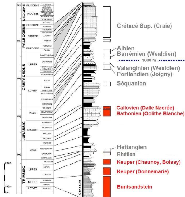
Fig. 1- Selection of the stratigraphic target suitable for CO 2 storage. Buntsandstein sandstones, Donnemarie, Chaunoy and Boissy sandstones (Keuper) and Dogger limestones. These targets are represented on the Paris Basin log (modified from Guillocheau et al., 2000 [8]).
