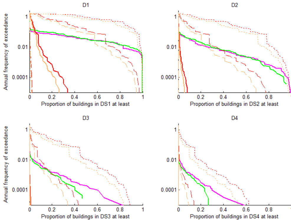
Figure 3. Mean annual frequencies of attaining or exceeding different damage states computed using fragility curves (magenta lines), fragility surfaces (green lines) and vulnerability indices (solid red and orange: best-estimate, dashed: plausible range and dotted: upper and lower bounds).
