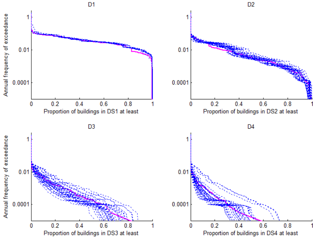
Figure 1. Annual frequencies of attaining or exceeding different damage states computed using fragility curves accounting for variability in the mechanical properties (dashed blue lines) and mean annual frequency (solid magenta lines), where DS1 corresponds to slight damage and DS4 corresponds to collapse.
