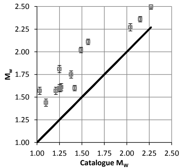
Figure 4: Comparison of moment magnitude ( M_w ) versus catalogue (a) local magnitude ( M_l ) and (b) moment magnitude ( M_w ) for the Hengill dataset. The Swiss M_l:M_w model is that of Goertz-Allmann et al. (2011).
