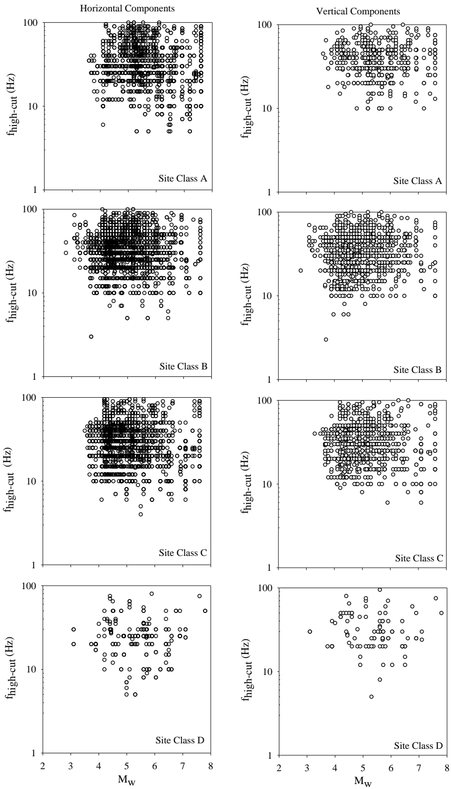
Figure 13. Same as Figure 12 but for high-cut filter frequencies.
