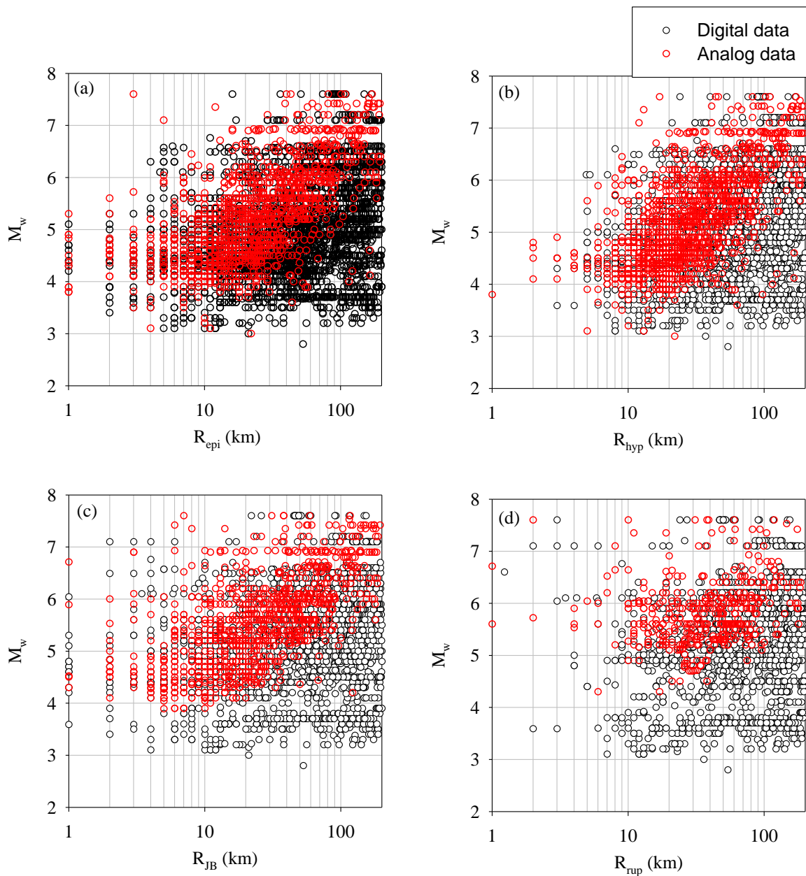
Figure 11. Distribution of M_w vs. (a) R_{epi} , (b) R_{hyp} , (c) R_{JB} and (d) R_{rup} . Scatter points in red color indicate analog records whereas black scatter points designate digital records. Moment magnitude information given on each plot is either directly extracted from the original reference source (see Tables A1 and A2) or estimated from an empirical relationship as explained under the “Compilation of Earthquake and Strong-Motion Station Metadata” subsection.
