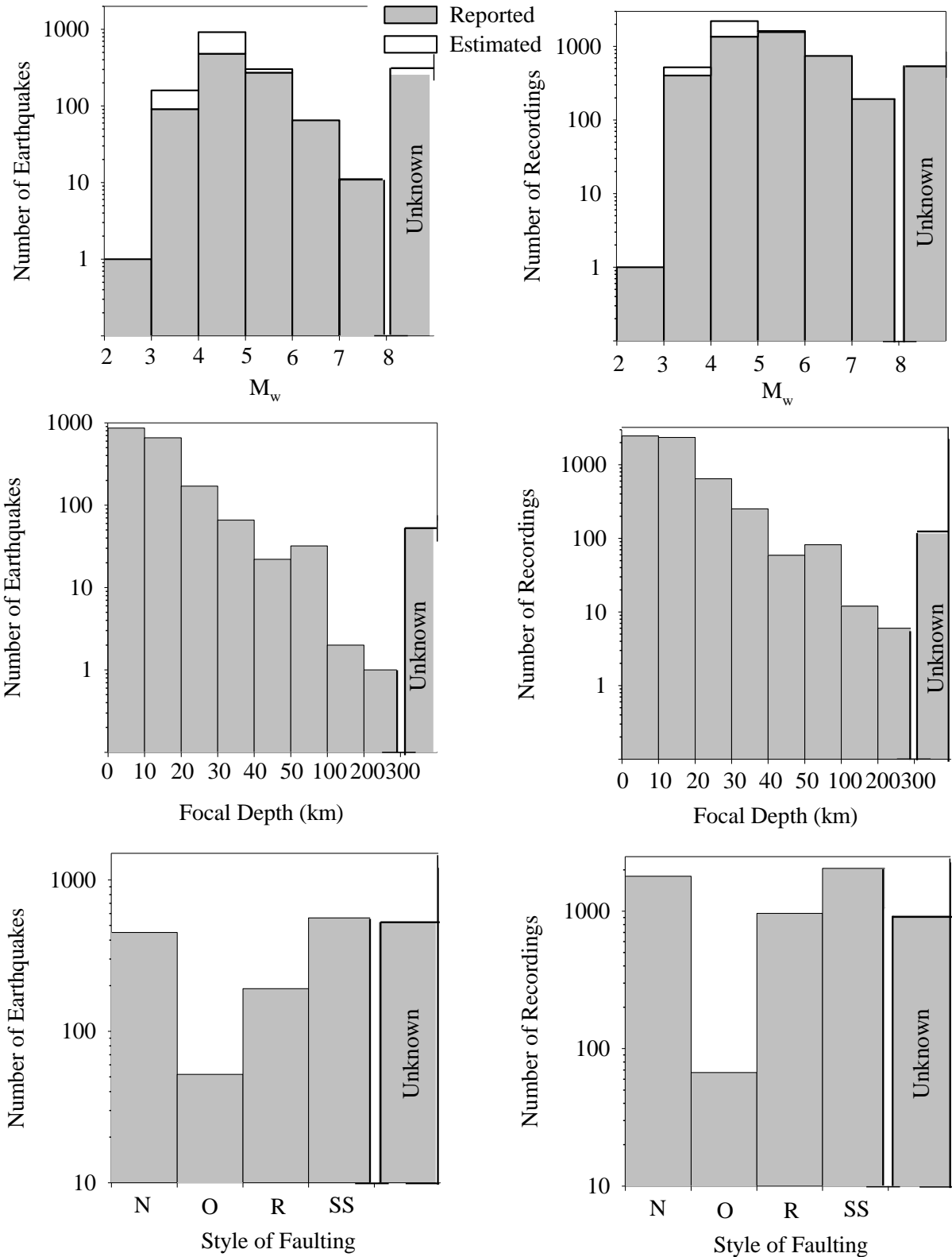
Figure 9. Distributions of events (first column) and accelerograms (second column) in RESORCE in terms of moment magnitude (first row), depth (second row) and SoF (third row). The vertical bars labeled as “Unknown” refer to the events or accelerograms that cannot be classified within any one of these parameters due to missing event or strong-motion station metadata information.
