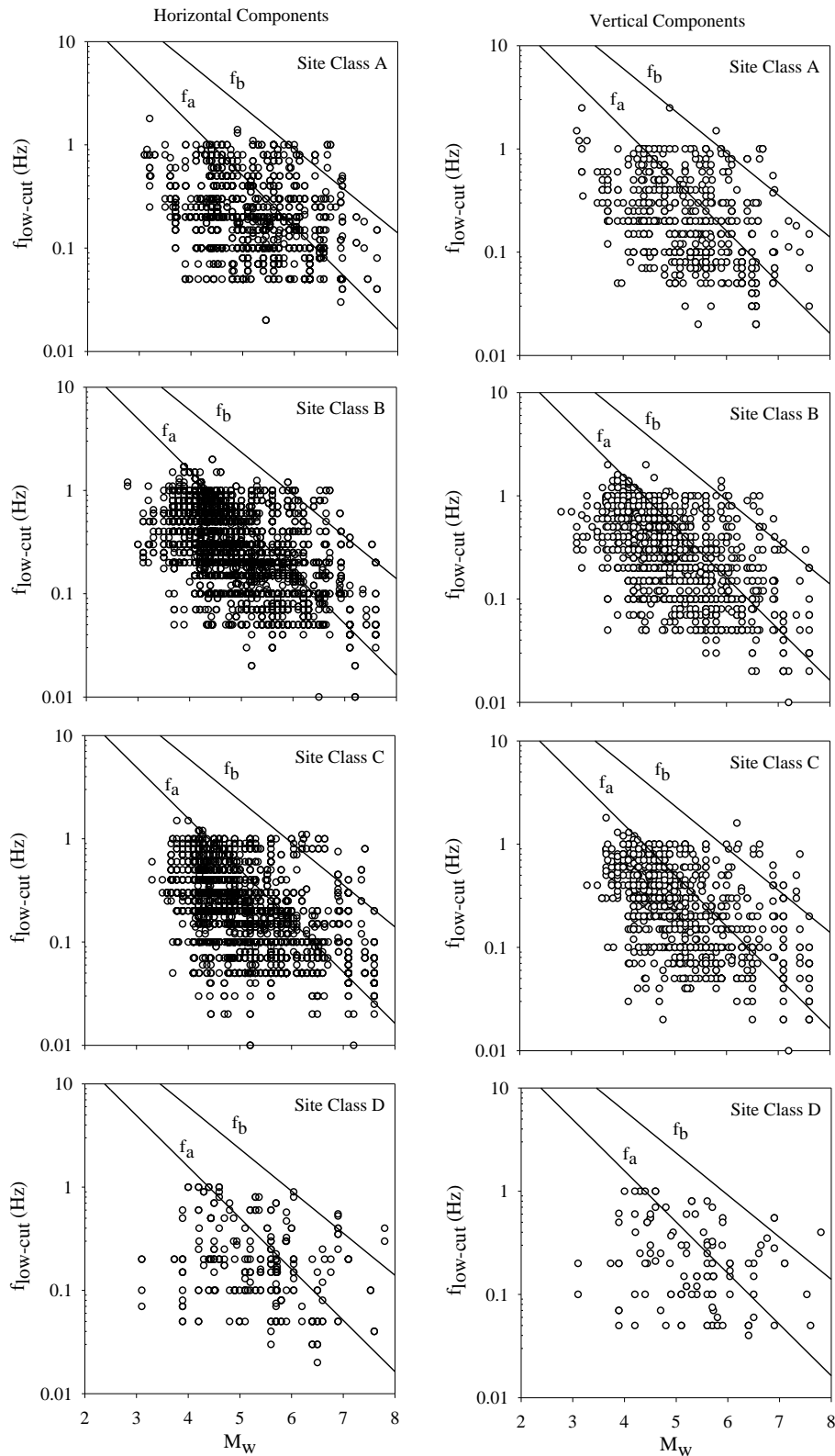
Figure 12. Variation of low-cut filter frequencies as a function of M_w for different site classes in RESORCE. Moment magnitude information given on each plot is either directly extracted from the original reference source (see Tables A1 and A2) or estimated from an empirical relationship as explained under the “Compilation of Earthquake and Strong-Motion Station Metadata” subsection.
