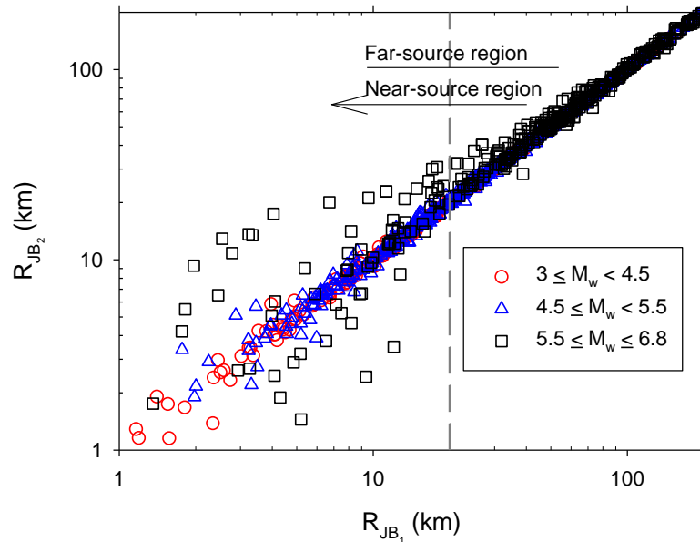
Figure 2. Differences between R_{JB_1} - R_{JB_2} pairs computed from the two planes given by the double-couple fault-plane solutions in the absence of extended-source distance measures ( R_{JB} and R_{rup} ) in the reference source databases. Different color codes and symbols indicate different magnitude intervals.
