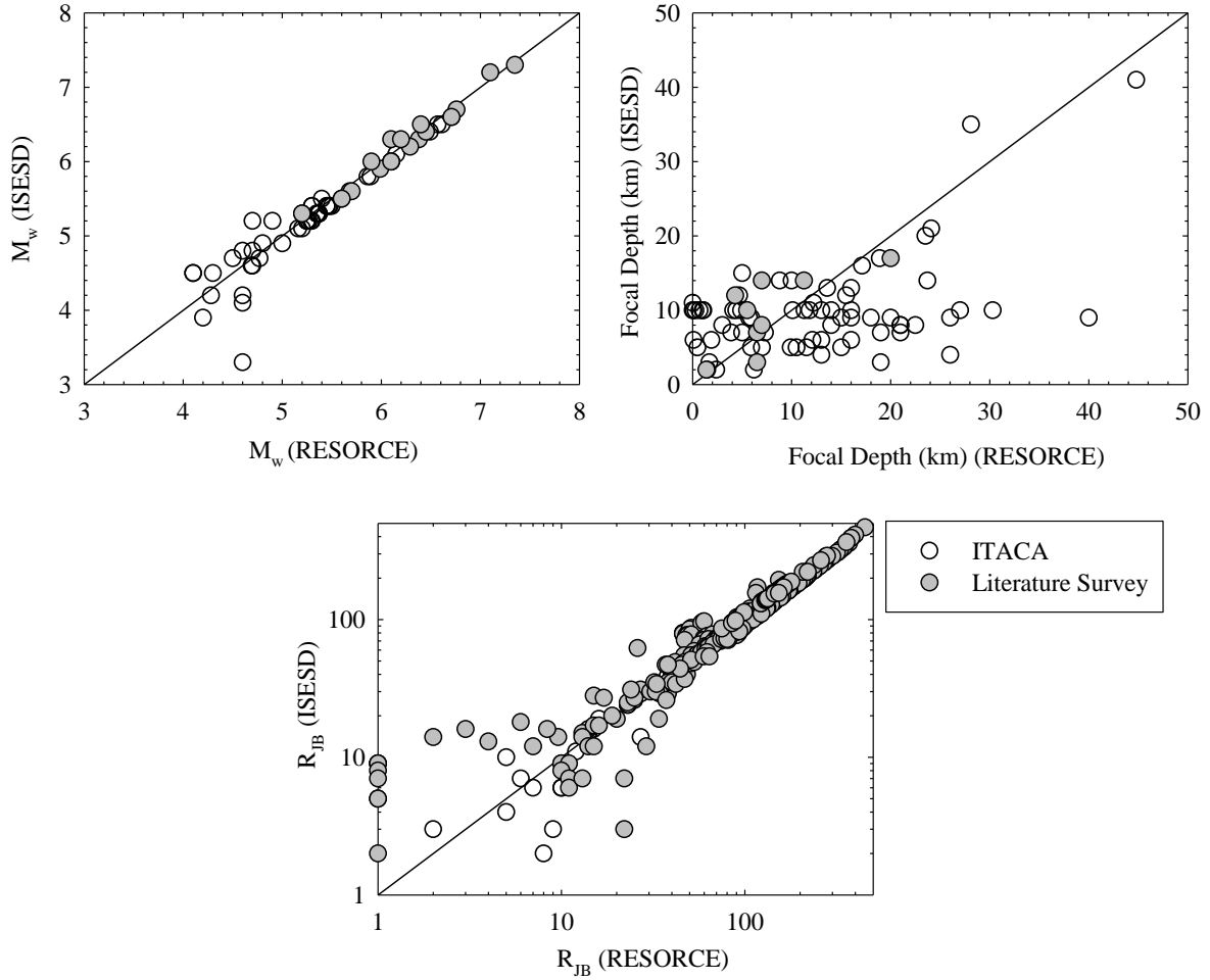
Figure 5. Differences in moment magnitude ( M_w ), focal depth and source-to-site distance information before and after updating the ISESD strong-motion databank by following the strategy outlined in the previous section. (Grey circles show the modifications based on recent literature survey. White circles denote the modifications due to ITACA).
