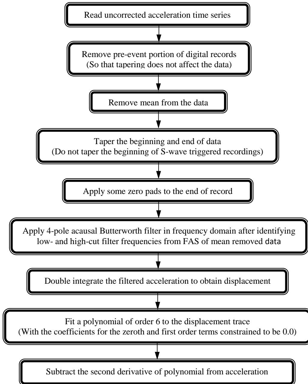
Figure 4. Band-pass filtering and post-processing scheme (after the removal of existing non-standard errors) used in RESORCE (modified from Boore et al., 2012). The original version of the implemented procedure is given in Chiou et al. (2008).
