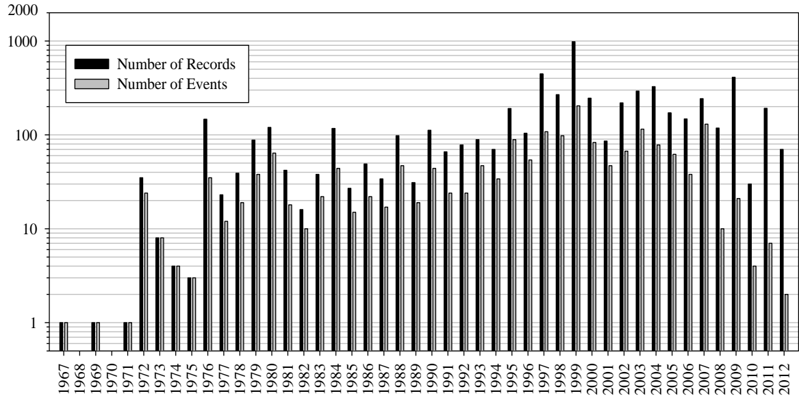
Figure 7. Annual distribution of accelerograms and earthquakes in RESORCE
