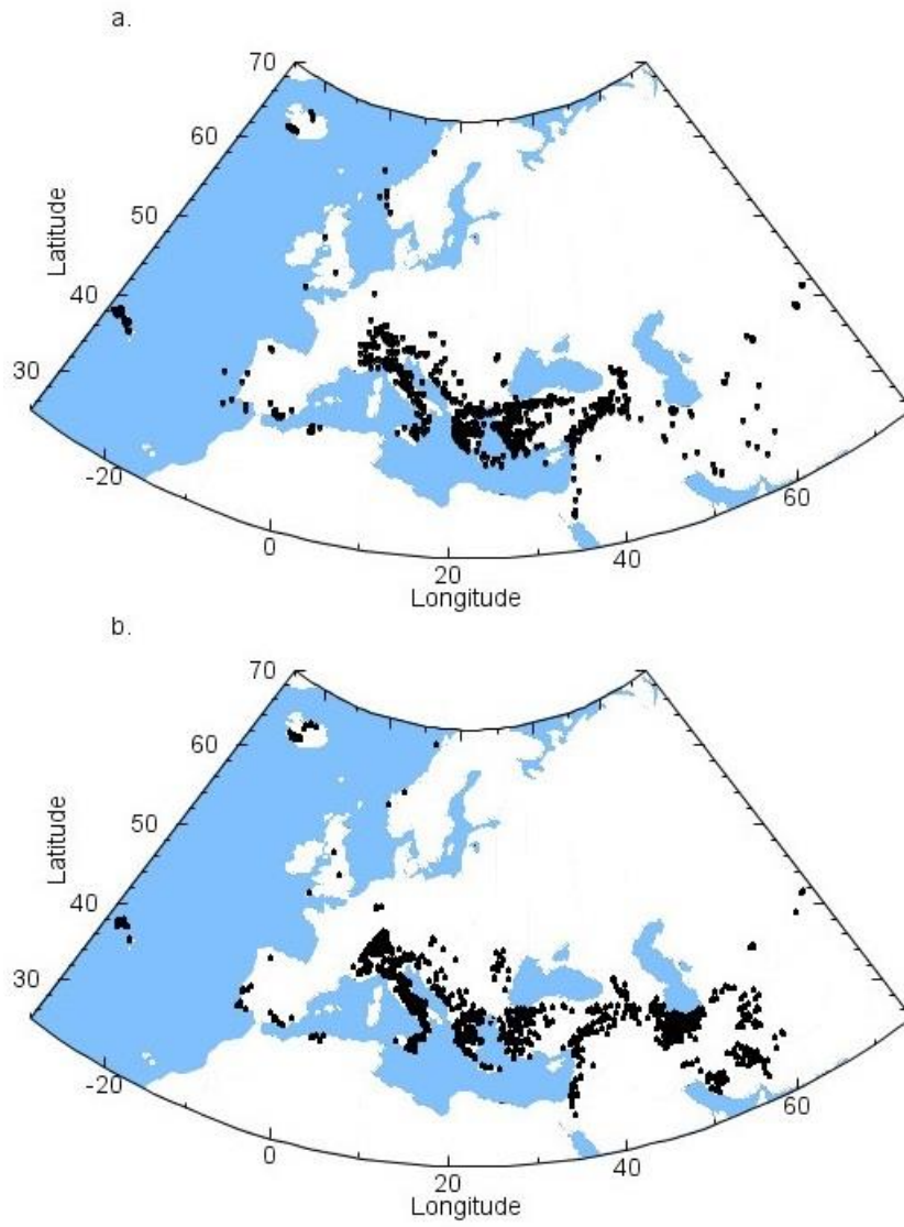
Figure 8. Geographical distributions of (a) earthquakes and (b) strong-motion stations in RESORCE
