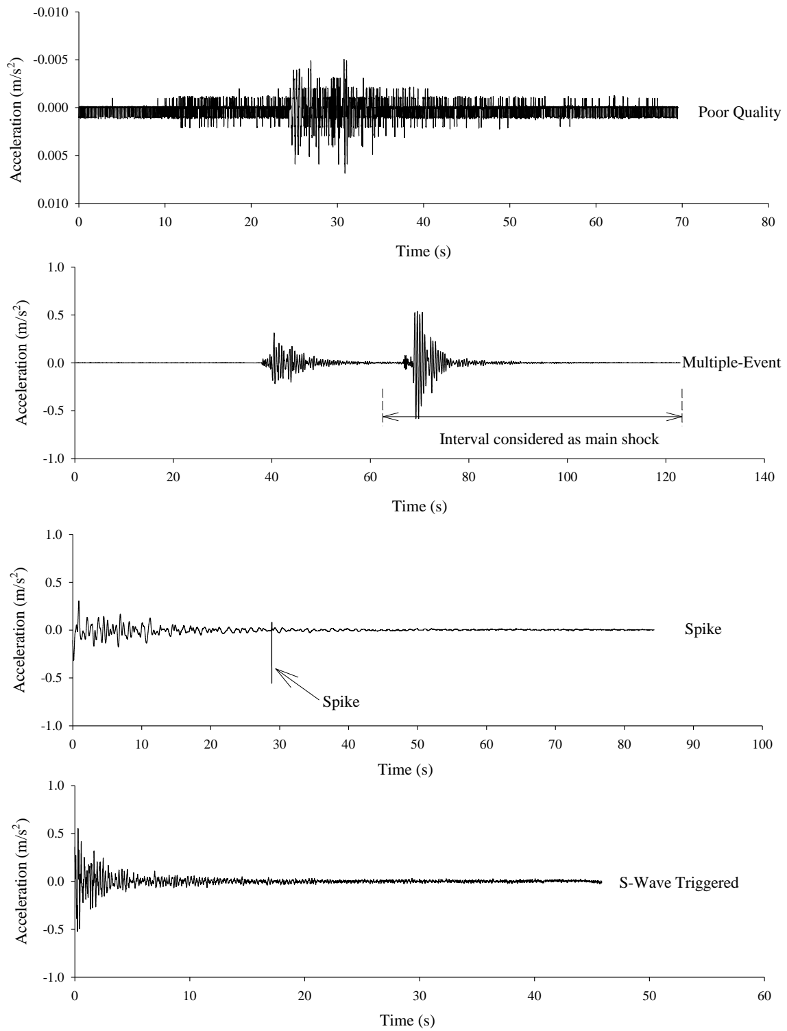
Figure 3. Example waveforms featuring different types of non-standard errors in time domain.
