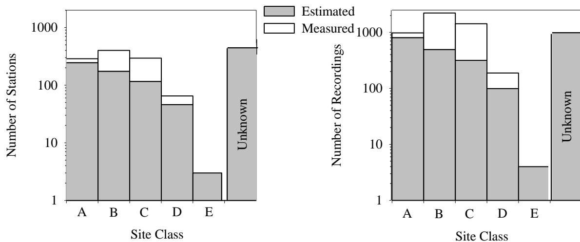
Figure 10. Distributions of strong-motion stations (left panel) and accelerograms (right panel) in RESORCE in terms of Eurocode 8 (CEN, 2004) site classes. The explanation about the labels designated as "Unknown" is similar to the one given in the caption of Figure 9.
