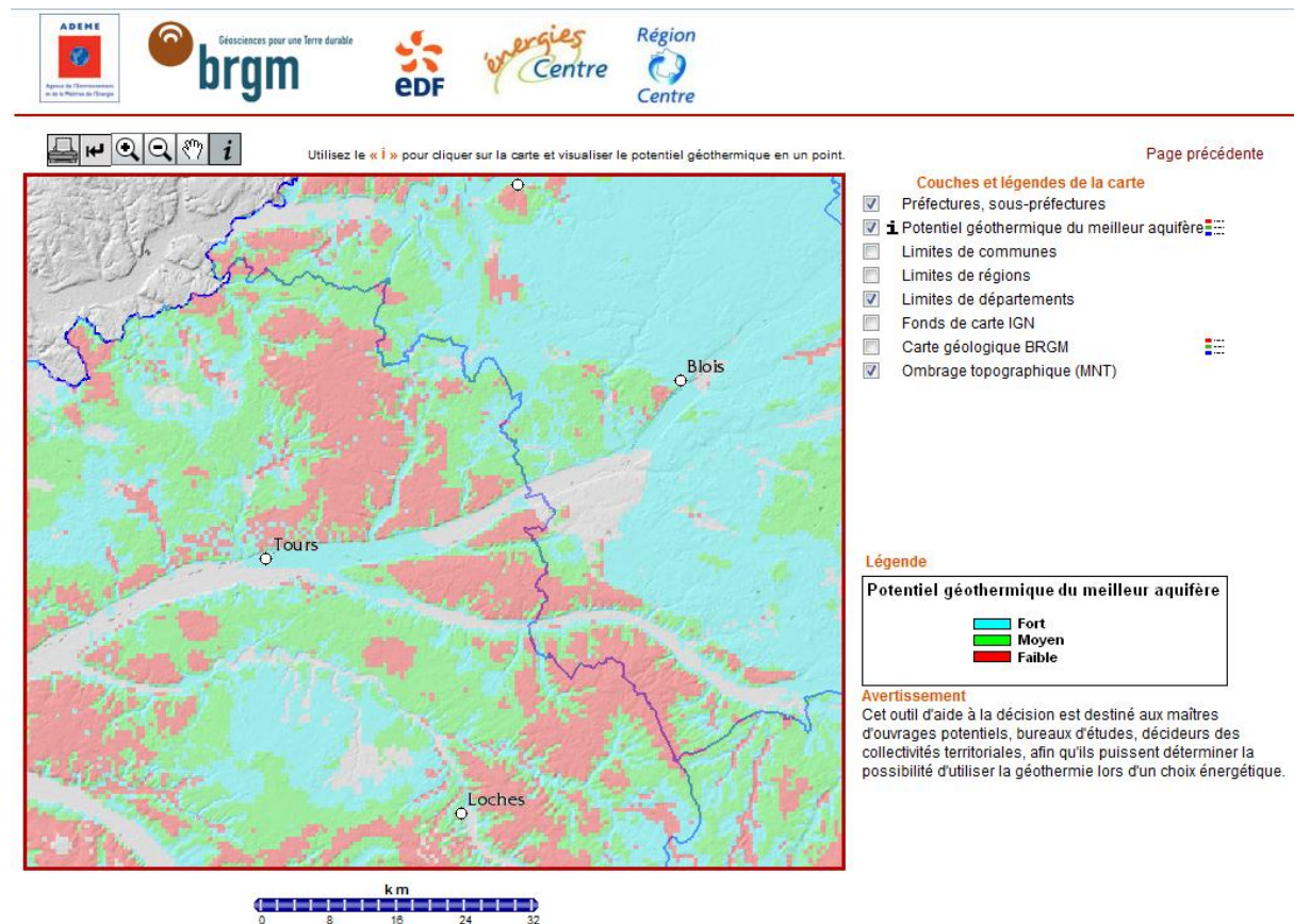
Figure 2: GIS for the geothermal potential of shallow aquifers in France, dedicated to the general public (ADEME-BRGM). Zoom on the “région Centre”. Colours indicate a qualitative geothermal potential combining the estimated flow rate and depth of the aquifer: High (blue), Medium (green) and Low (red).
