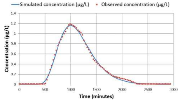
Figure 13. Observed and computed breakthrough curve using Eq. (18) (Radial converging flow).
