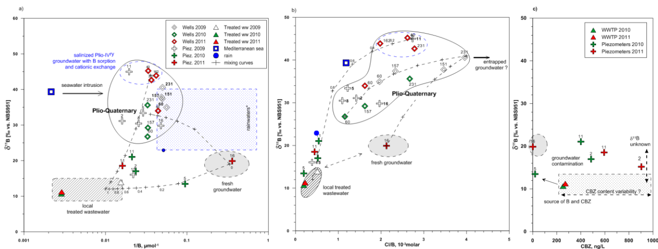
Figure 5: a) \delta^{11}\text{B} versus 1/\text{B} in samples from the wells, piezometers, and wastewater recharge plant during the three years. b) Boron isotopic composition versus the 10^{-3} molar ratio \text{Cl}/\text{B} , (c) Boron isotopic signatures versus carbamazepine concentrations for piezometer samples in 2010 and 2011. The \delta^{11}\text{B} of Piez 2 in 2011 was not measured. Error bars are within the points. The boron isotopic compositions and rainwater concentrations* are taken from Millot et al. (2010). All mixing curves were calculated using binary mixing lines according to Faure (Faure, 1986).
