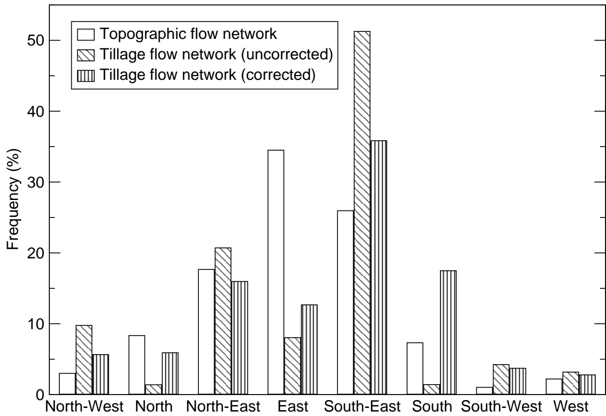
3 Fig. 10. Distribution of the flow directions for the computed flow networks.
