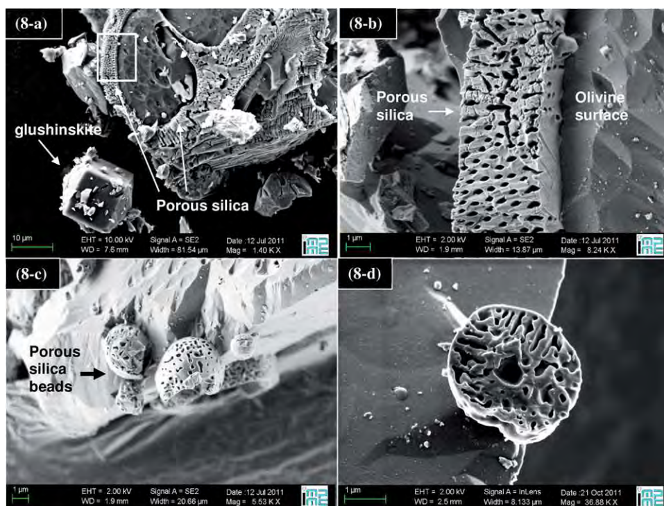
Fig. 8. FEG-SEM images of solid particles after 1 h of reaction ( 3 \text{ g l}^{-1} slurry with 0.1 \text{ M} oxalate salt, under 120^\circ\text{C} and 20 \text{ bar} of \text{CO}_2 ). (a) An olivine particle partially covered by a porous silica layer; glushinskite crystals are observed. (b) The microstructure of the highly porous precipitated silica layer. (c and d) Micrometric porous silica beads on the olivine surface.
