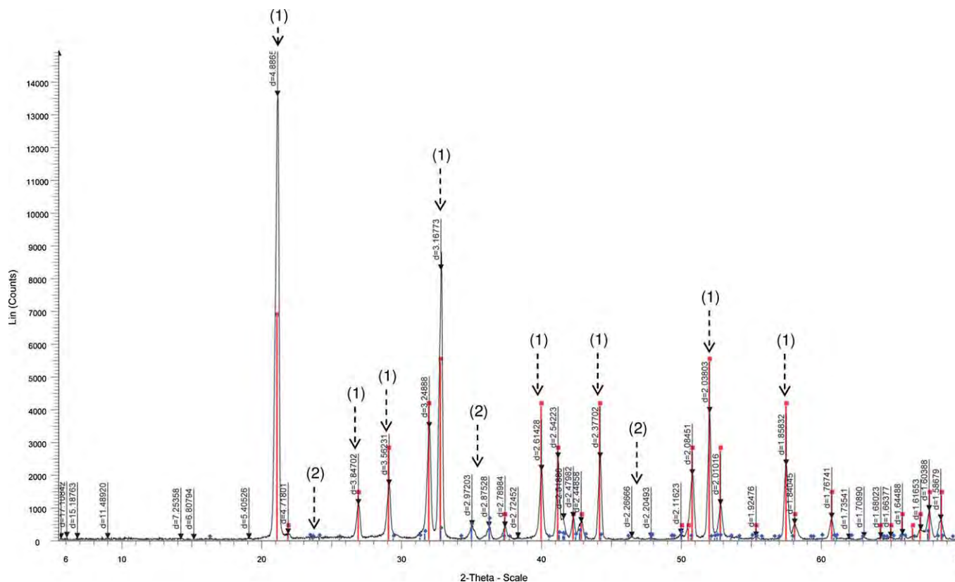
Fig. 4. X-ray diffraction pattern of final solid product under dilute slurry conditions ( 3 \text{ g l}^{-1} of olivine with 0.1 \text{ M} disodium oxalate, 120^\circ\text{C} and 20 \text{ bar} of \text{CO}_2 ). (1) \alpha\text{-MgC}_2\text{O}_4 \cdot 2\text{H}_2\text{O} (23-0394) or synthetic glushinskite, (2) clinoenstatite (35-0610) (traces) from initial material.
