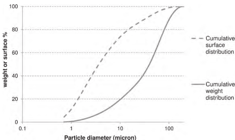
Fig. 2. Cumulative particle size distribution by mass and by surface for ground olivine sieved under 100 µm.
