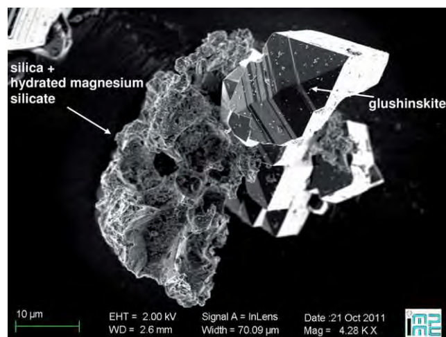
Fig. 9. FEG-SEM image of solid particles after 24 h of reaction ( 3 \text{ g l}^{-1} slurry with 0.1 \text{ M} oxalate salt, under 120^\circ\text{C} and 20 \text{ bar} of \text{CO}_2 ).
