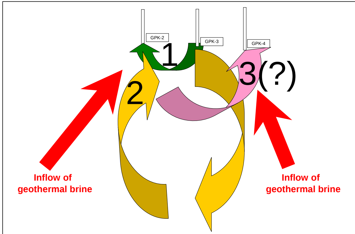
Figure 3 - Conceptual model of fluid circulation in the Soultz geothermal heat exchanger established after the 5 month-circulation test carried out in 2005 (injection rate into GPK-3 close to 15 l/s, with 11.9 l/s coming from GPK-2 and 3.1 l/s from GPK-4) and the associated tracer test using fluorescein (after Sanjuan et al., 2006b). 1) Short-scale loop between GPK-3 and GPK-2 (fluorescein recovery rate of 15.6%; mean linear fluid velocity of 1.1 m/h). 2) Large-scale loop between GPK-3 and GPK-2 (fluorescein recovery rate of 7.9%; mean linear fluid velocity of 0.3 m/h). 3) Hydraulic connection between the large-scale loop and GPK-4 (fluorescein recovery rate of 1.8%; mean linear fluid velocity of 1.1 m/h). The existence of another quasi-infinite loop, which would connect both GPK-2 and GPK-4 to GPK-3, is highly probable. The presence of such a loop could explain the low fluorescein recovery rate estimated at the end of the tracer test ( 15.6 + 7.9 + 1.8 = 25.3\% ). The omnipresence of the native geothermal brine (with a natural flux estimated at 1\text{--}1.2\text{ m}^3/\text{h} ) was observed in the three deep wells during all the production and circulation tests carried out after 2000. Similar (or slightly lower) mean linear fluid velocities (0.25–0.45 m/h) and tracer recovery rate (26%) were obtained between GPK-1 and GPK-2 at 3500–3900 m depth during the 4 month 1997 circulation test when 21 to 25 l/s injection rates were used (Vaute, 1998; Aquilina et al., 2004).
