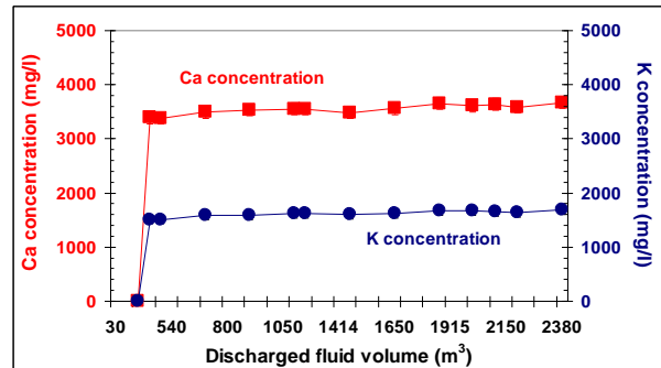
Figure 5 - Concentrations of dissolved K and Ca analyzed in the fluid discharged from the well GPK-4 between January 22 and 25, 2007.
