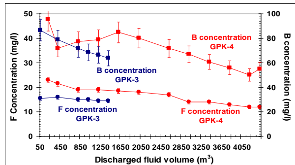
Figure 10 - Concentrations of dissolved F and B analyzed in the fluids discharged from GPK-3 and GPK-4 in February and March 2007.
