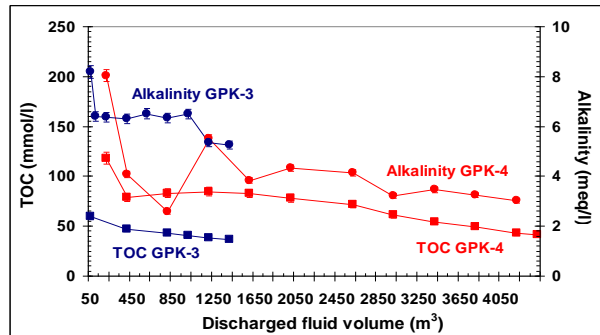
Figure 9 - Concentrations of TOC and alkalinity values determined in the fluids discharged from GPK-3 and GPK-4 in February and March 2007.
