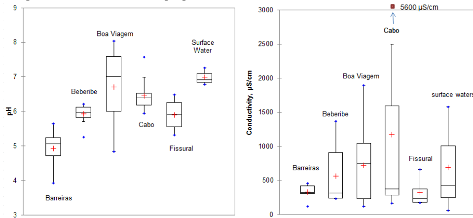
Figure 2: Box plots of pH and EC measured on site during the first sampling campaign in September 2012.
