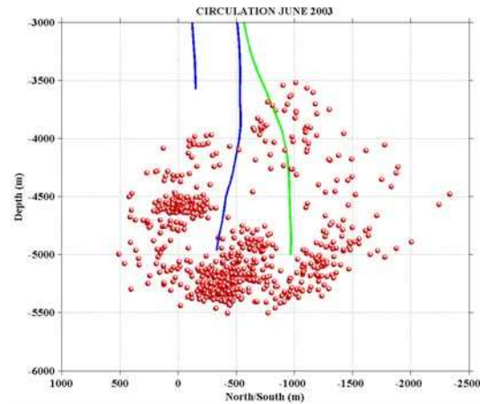
Figure 4: Microseismic events generated during the circulation test between GPK2 & GPK3
