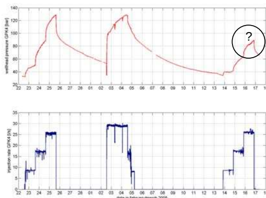
Figure 11: Pressure and flow for the acidization test
