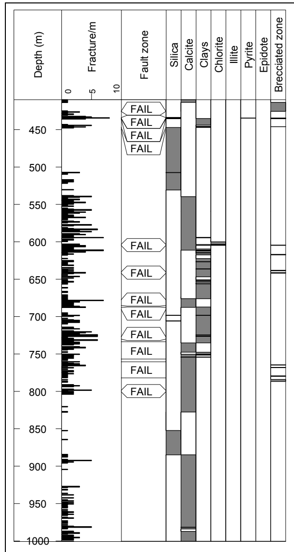
Figure 7. Fracture density, major fault location, and vertical distribution of the hydrothermal fillings sealed fractures in the Californiae well.
