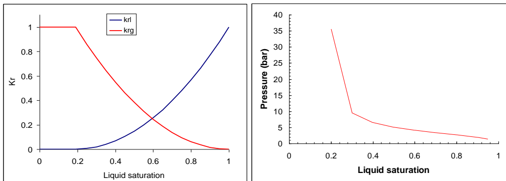
Figure 4 Relative permeability and capillary pressure curves according to liquid saturation ( S_l ).
