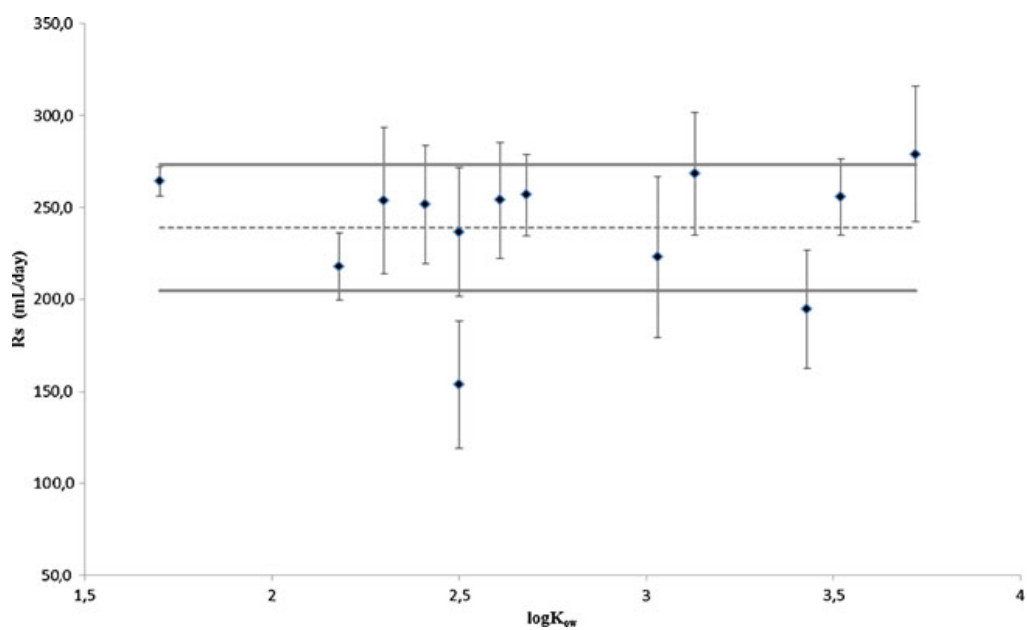
Fig 3 Average sampling rate of POCIS for pesticides whose polarity varies from 1.7 to 3.7. Discontinuous line of the figure represents the mean Rs value. Continuous lines represent the 20 % of RSD calculated from the 13 Rs values
