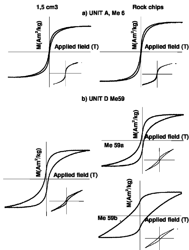
Figure 9. Comparison of hysteresis loop shapes between the 1.5 cm 3 samples and the subsampled rock chips. Distribution of iron oxide phases is homogeneous in unit A and heterogenous in unit D.
