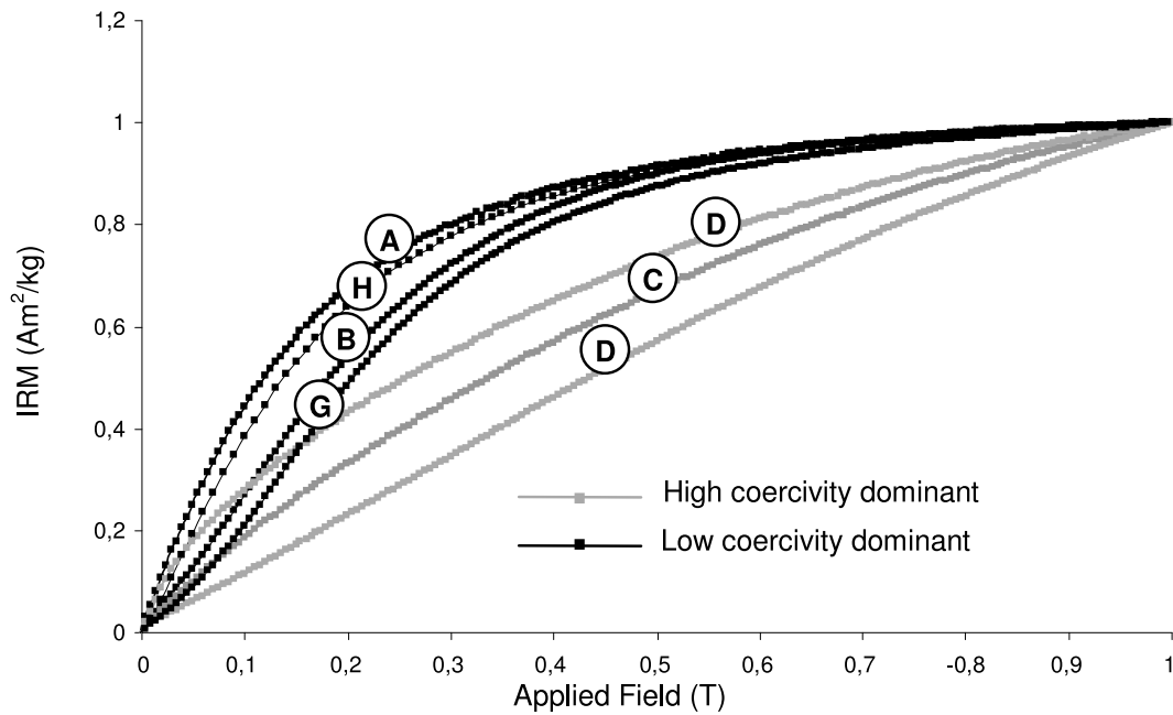
Figure 7. Isothermal remanent magnetization (IRM) curves on representative samples from the Les Mottes section. Letters refer to section units (see Figure 3). Representative curves have been normalized at 1 T.
