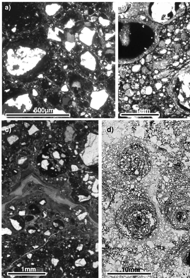
Figure 4. Micromorphology of red siderolithic formations in the Les Mottes section: (a) Granules with quartz grain cores encapsulated in ferruginous cortex (cross-polarized light). (b) Bleaching of granules in the mottled unit (plane-polarized light). (c) Pedotubule with granule infillings and illuviation cutans (plane-polarized light). (d) Nodular silcrete at the top of the section, the nodules show increasing envelopes with clear geotropism, matrix is silicified (plane-polarized light).
