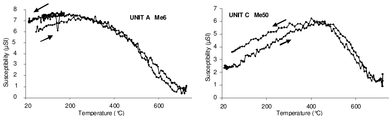
Figure 6. Susceptibility versus temperature for representative samples of the Les Mottes section units A and C. The gradual decrease in susceptibility, which shows an ordering temperature at \sim 650^\circ\text{C} , reveals the presence of haematite.
