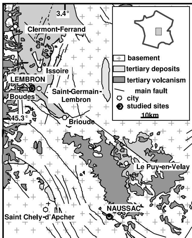
Figure 1. Geological sketch of the central part of the French Massif Central. The siderolithic formations outcrop at the edge of the Tertiary grabens. Volcanic flows cover these deposits. Sampled sites are indicated in capital letters.
