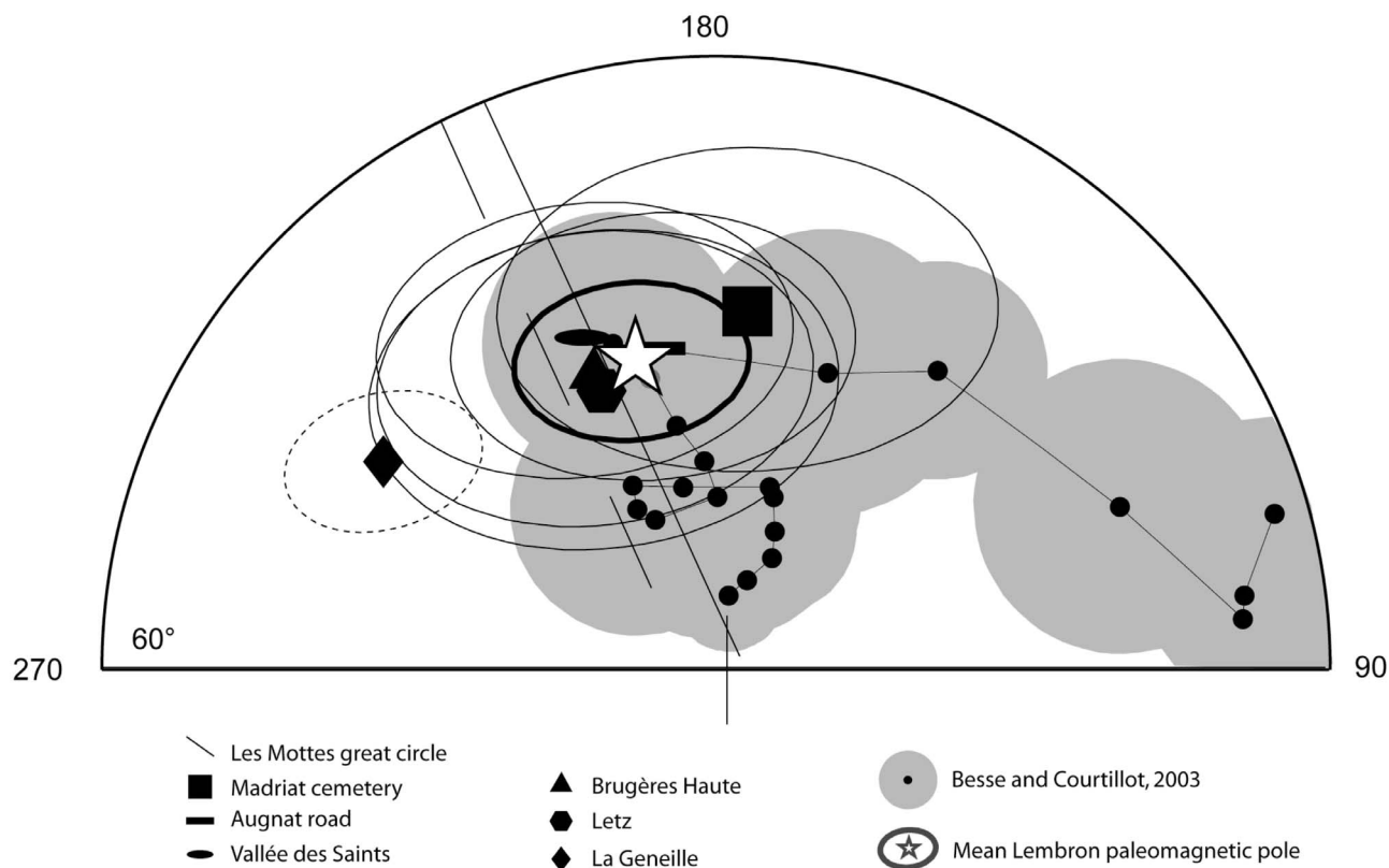
Figure 15. Paleomagnetic poles obtained in the Lembron area compared to the 0–200 Ma APWP of Eurasia [Besse and Courtilot, 2003]. McFadden [1982] test is negative comparing “La Geneille” Paleomagnetic pole and mean Lembron paleomagnetic pole. Mean paleomagnetic pole is close to the 140 Ma pole of the Eurasian APWP.
