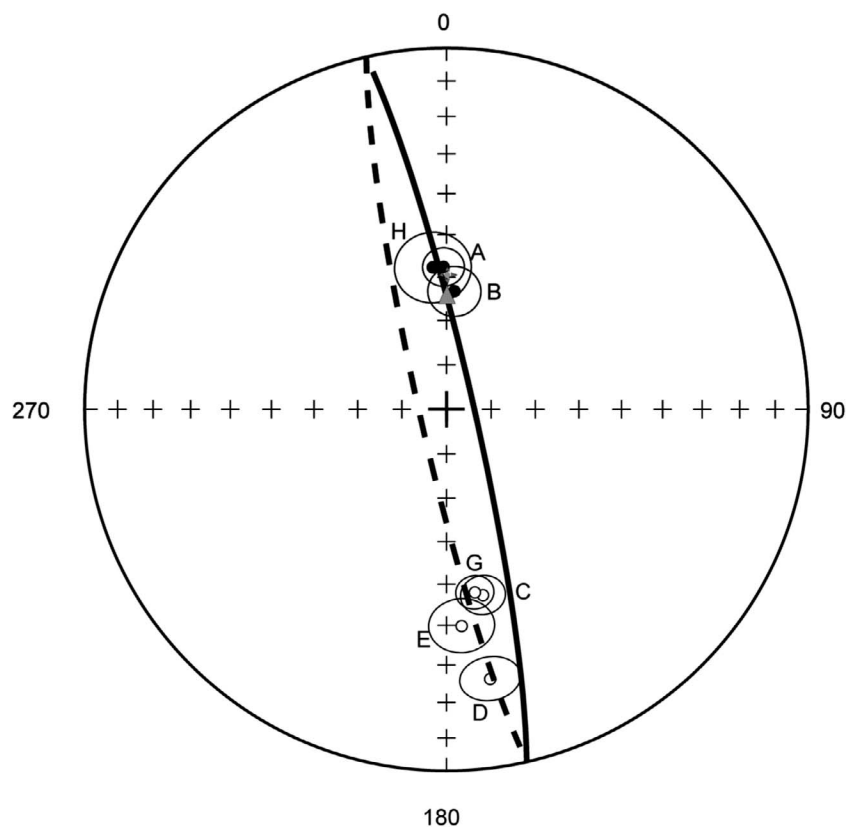
Figure 12. Equal-area projection of mean characteristic directions for Les Mottes units. Directions are fitting a great circle. Small stars represent the mean direction with its 95% confidence circle. Closed (open) symbols refer to directions in the lower (upper) hemisphere. Grey crosses represent the IGRF (declination: -0.7^\circ ; inclination: 61.2^\circ ) and grey triangles the GAD (Inclination: 63.8^\circ ).
