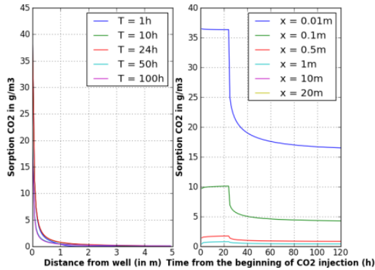
Figure 7. Evolution of CO 2 adsorbed, function of space (on left) and of time (on right)
