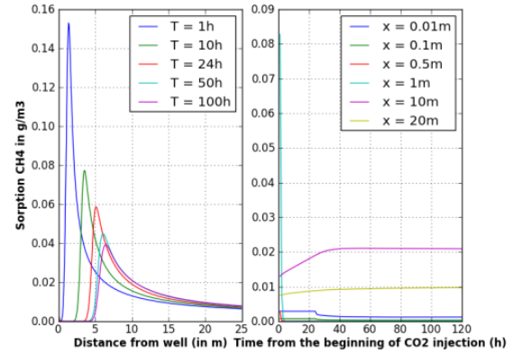
Figure 8. Evolution of CH 4 adsorbed, function of space (on left) and of time (on right)
