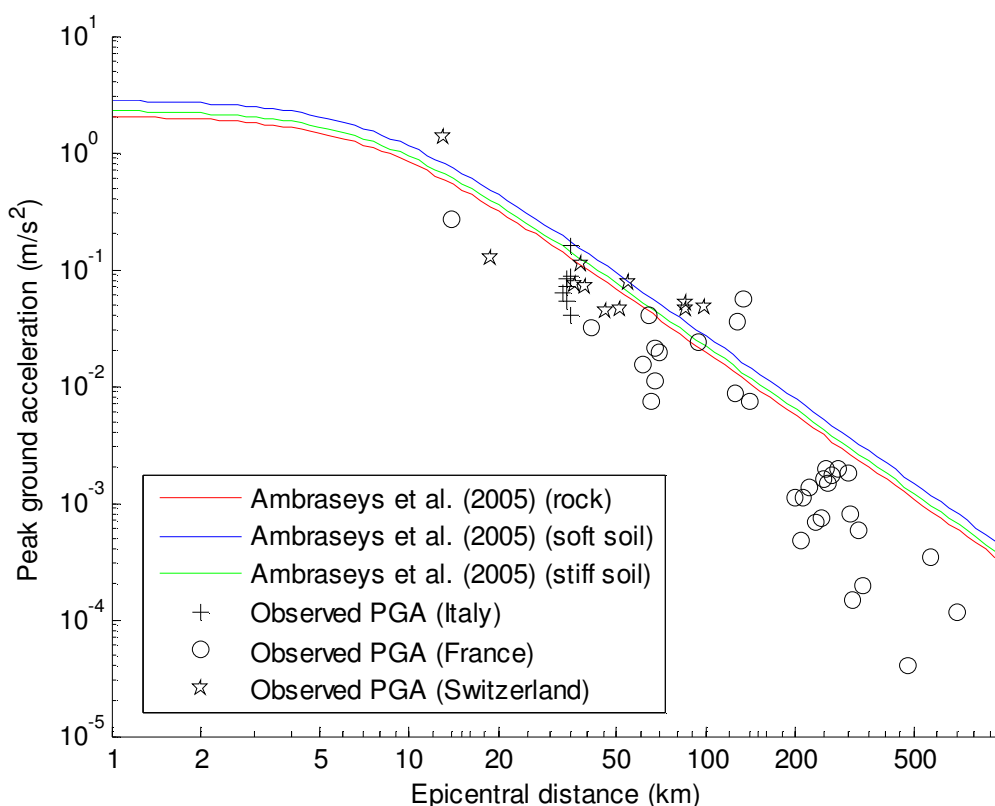
Figure 4. Comparison between the peak ground accelerations recorded during the Vallorcine earthquake (Mw 4.5, strike-slip mechanism) and the values predicted by the ground-motion model of Ambraseys et al. (2005).
