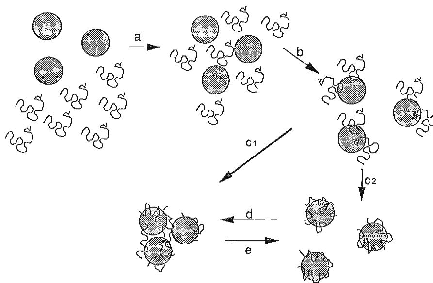
Fig. 5 - Mode of action and conformation of organic coagulants with the particle surface.
