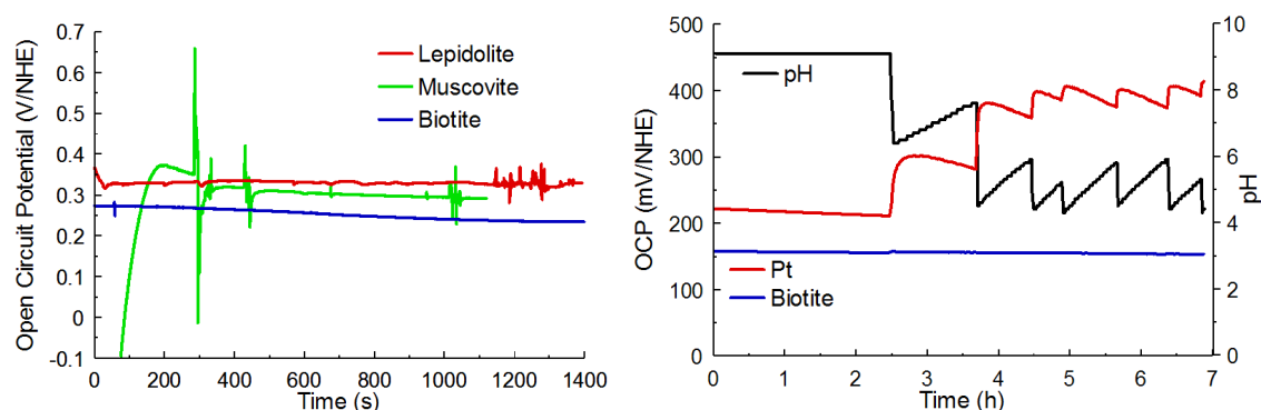
Figure 1: (left) OCP measurements recorded after immersion of various electrodes in NaCl 0.1M (pH 7.5). (right) Effects of HCl 0.1M repeated dropwise addition in the bathing electrolyte on a biotite electrode and on a platinum electrode.
