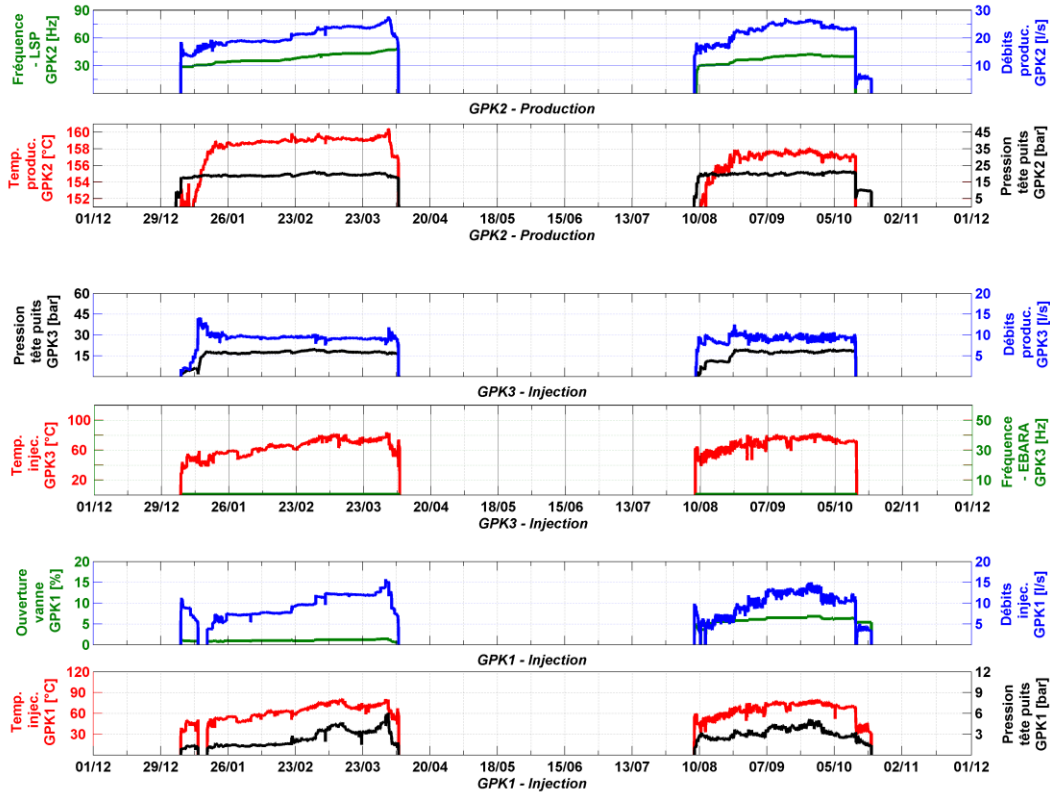
Figure 4: Overview of flow rates (blue), wellhead pressures (black) and temperatures (red) for the Soultz wells GPK-1, GPK-2, and GPK-3 during hydraulic circulation in 2011. Also shown in green are the frequencies of the production pump and injection pump (Ebara pump for GPK-3) and the aperture of the valve for re-injection into GPK-1.
