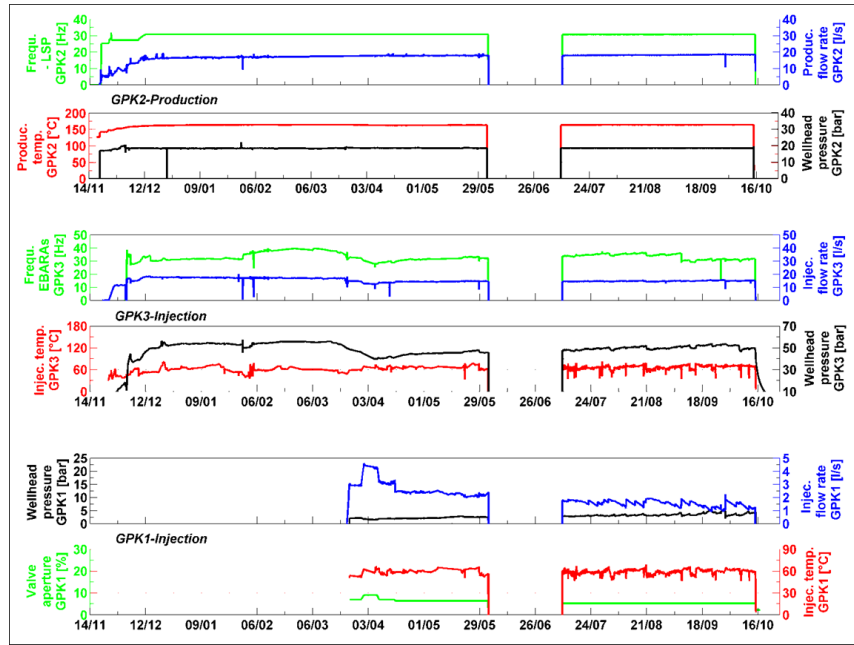
Figure 3: Overview of flow rates (blue), wellhead pressures (black) and temperatures (red) for the Soultz wells GPK-1, GPK-2, and GPK-3 during hydraulic circulation from November 2009 to October 2010. Also shown in green are the frequencies of the production and injection pump (Ebara pump for GPK-3) and the aperture of the valve for re-injection into GPK-1.
