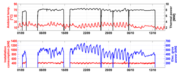
Figure 13: Thermal output of the Soultz plant in MWth and ambient air temperature versus time (above). Gross electrical power and self-consumption in kWe produced by the power plant versus time (below).
