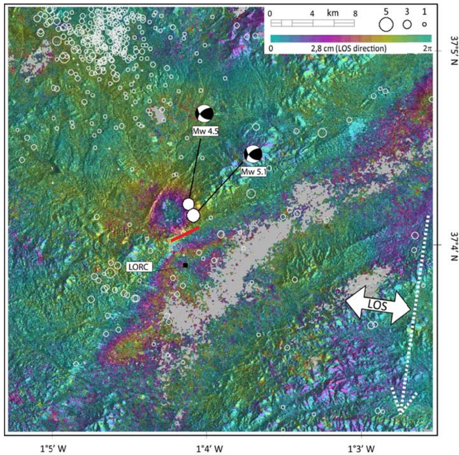
Figure 1: Surface displacement field due to both the Lorca earthquake and 5.2 month of water pumping in the Guadalentin basin. Empty white circles represent instrumental seismicity (IGN catalogue) and magnitude; full white circles represent the main shocks locations and magnitudes (IGN catalogue –please see López-Comino et al. (2012) for detailed aftershock relocation-). The main shocks, Mw 4.5 and Mw 5.1 on the 11 of May 2011 are plotted with their respective focal mechanism. One colour fringe corresponds to 2\pi phase cycle i.e. 2.8 cm in the Line of Sight (LOS) direction ( 23^\circ off the vertical). The red segment represents the surface extension of the modeled seismogenic fault.
