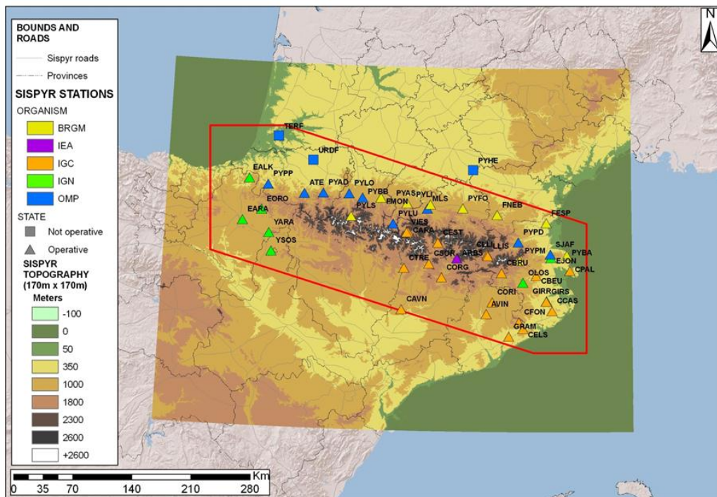
Figure 2 : Seismic stations sharing data on the NRT server (in red the limits of the area concerned by the Sispyr project)
