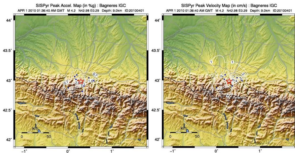
Figure 6 : Example of Pyrenean ShakeMap: PGA map with both ground motion and intensity input data. Preliminary results for 01/04/2010 event with M_l = 4.2 and GMPE Akkar & Bommer (2007)
