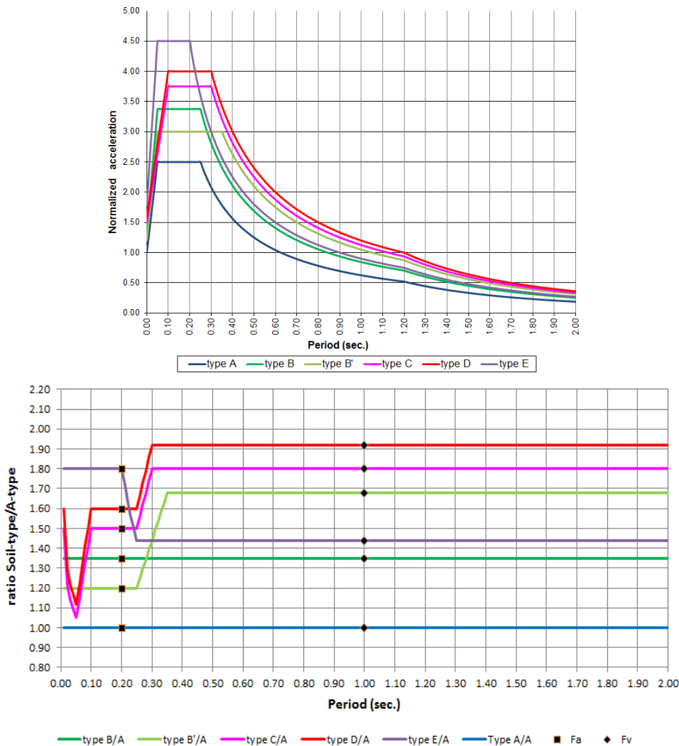
Figure 5: above: proposed normalized response spectra. Below: normalization of the response spectra with rock spectrum. Fa and Fv are deduced from ratio at period 0.2s and 1.0s
