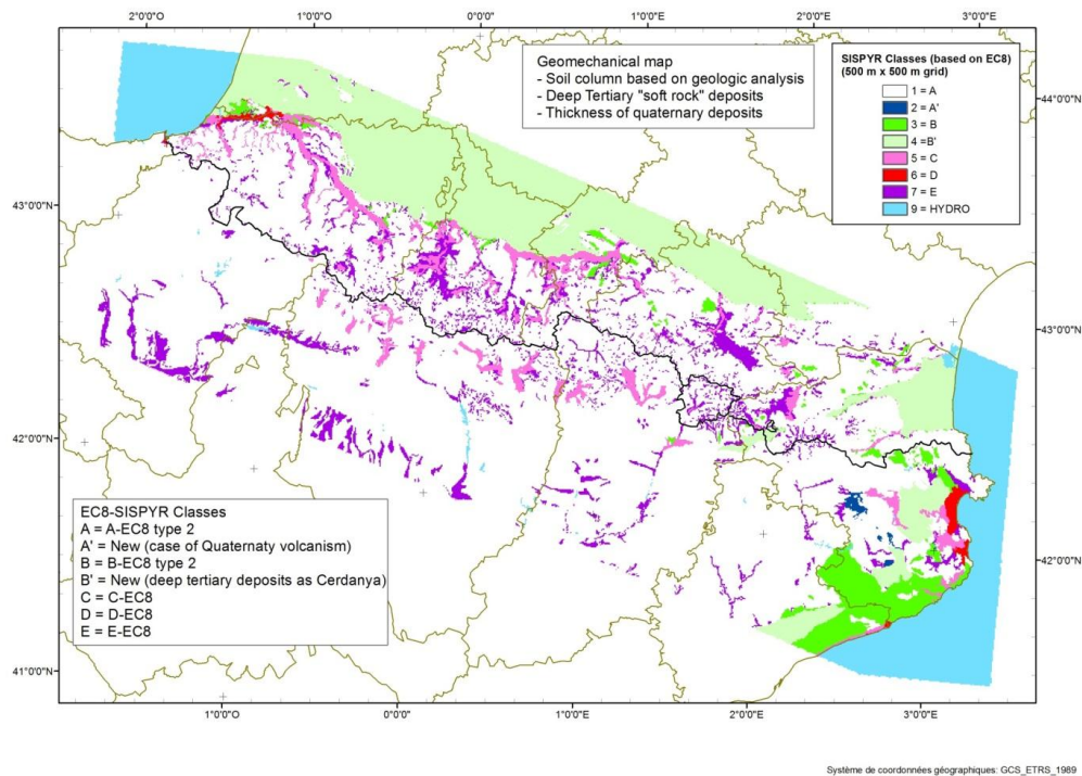
Figure 4: Site condition map based on EC8-type classes of soil
