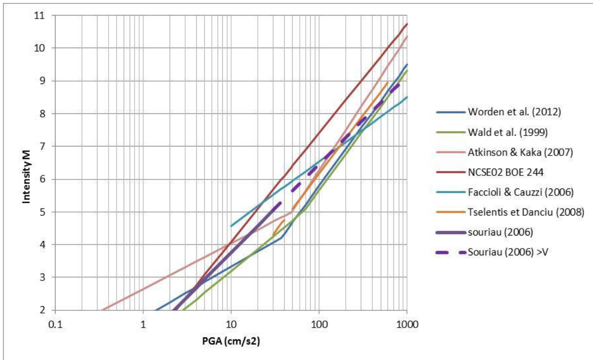
Figure 3: Comparison of GMICE that could be applied on ShakeMaps
