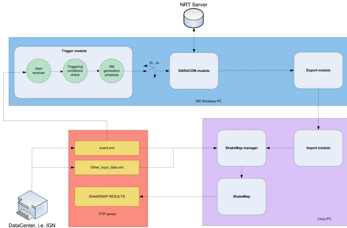
Figure 1. : Schematic diagram for the modules of the NRT process and their interconnection
