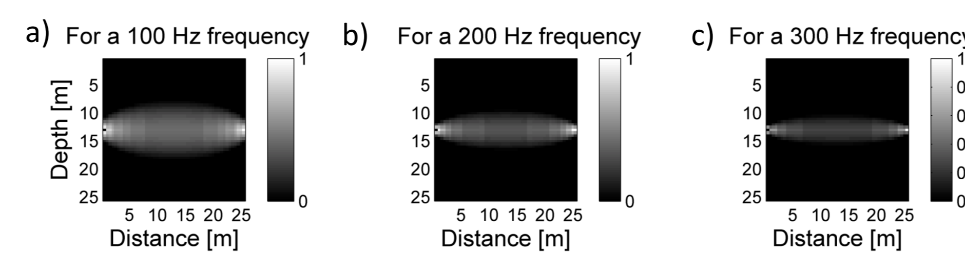
Figure 2 : Fresnel weights defined by Watanabe (1999) for different frequencies (Top) and sensitivity kernels used in the Quasi-Newton algorithm computed for different frequencies (Bottom)
