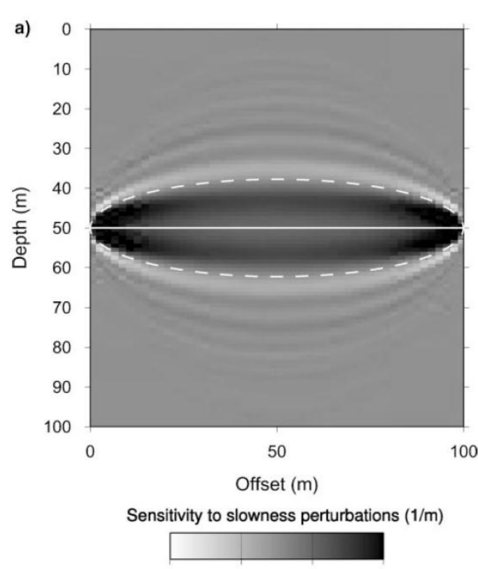
Figure 1 : 2D traveltimes sensitivity kernel for transmitted wave (Spetzler and Sniieder, 2004)
