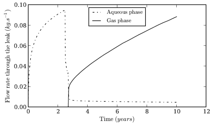
Figure 4: Brine and CO 2 leakage in the top aquifer during the 10 first years. Note the breakthrough of the gaseous phase at the date of 2.7 years.
