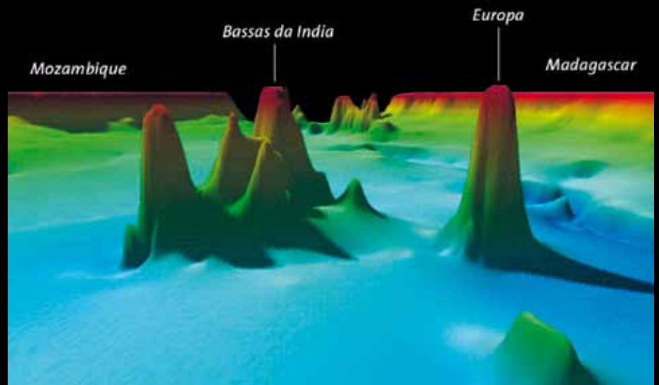
Fig. 6: Photos of the Bassas da India lagoon (the Scattered Islands of the Indian Ocean) and 3D view of bathymetry in the Mozambique Channel. © S. Jorry, Ifremer.
