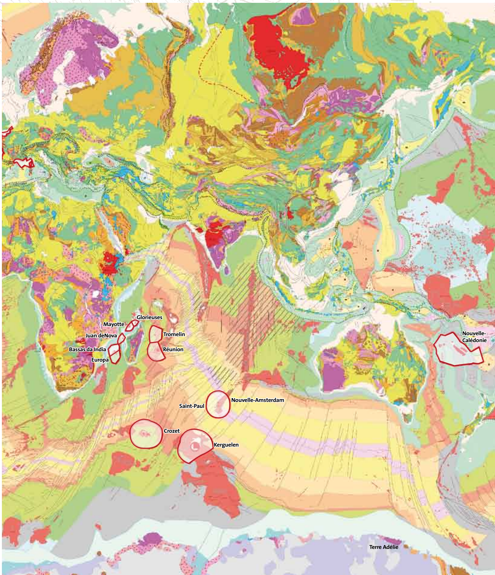
▲ Fig. 2: The geological map of the world showing the locations of the overseas territories and their exclusive economic zones (EEZ) including that of continental France (see the Extraplaç boxed text). Mercator projection. In the Pacific, Atlantic and Indian Oceans, yellows predominate, a colour chosen conventionally, representing geological age: the oceans are no older than 200 million years. Unlike the oceans, forever young, the oldest portions of the continents are some four billion years old. France's exclusive economic zone covers more than 10 million km 2 , the second largest in the world. The EEZ of the overseas territories corresponds to over 97% of this surface area, and that of Polynesia alone, amounting to 4.8 million km 2 , accounts for nearly half.
