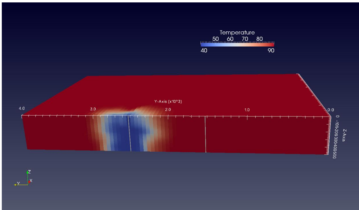
Figure 7: Cold plume extension after 10 years of geothermal exploitation (vertical wells positioned perpendicularly to channels, y direction).
