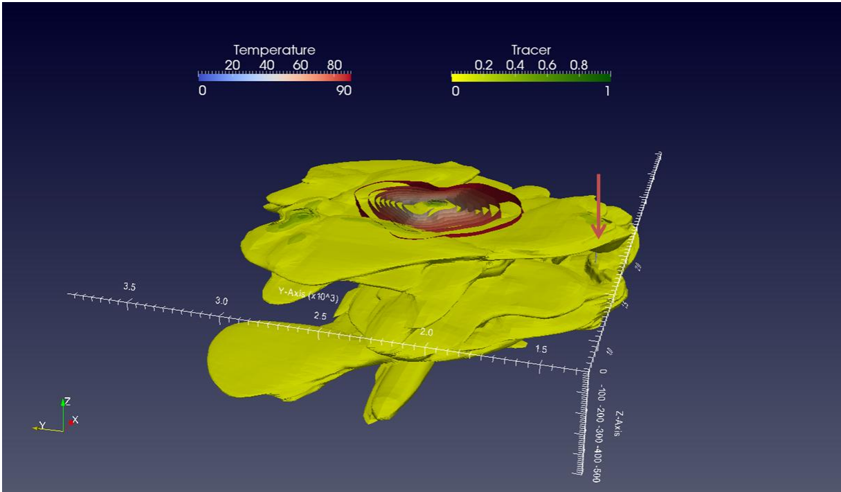
Figure 13: Temperature and tracer isocontours after 10 years of exploitation (vertical wells oriented according y direction).
