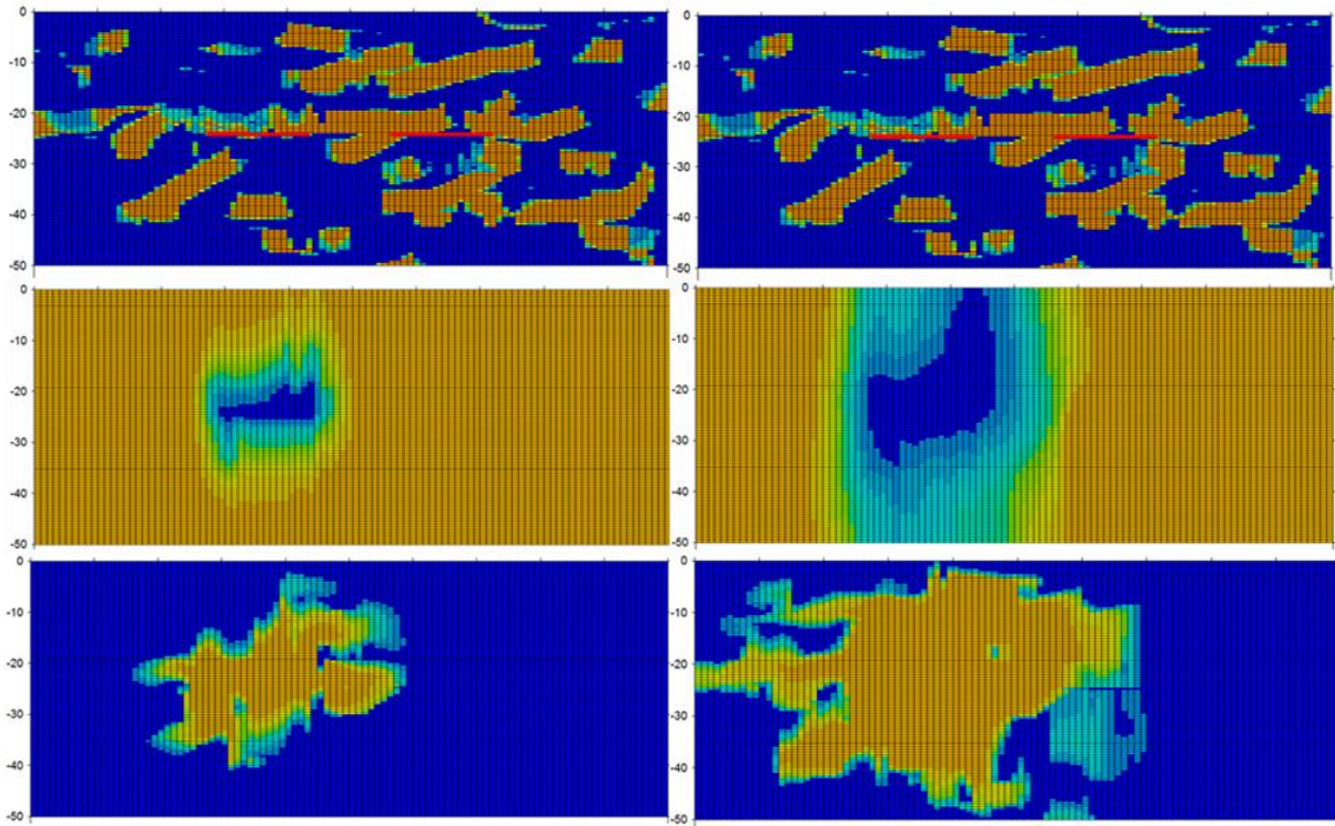
Figure 16: From top to bottom: horizontal permeability field and position of horizontal wells (red lines), temperature and tracer fields after 1 year (left) and 10 years (right)
