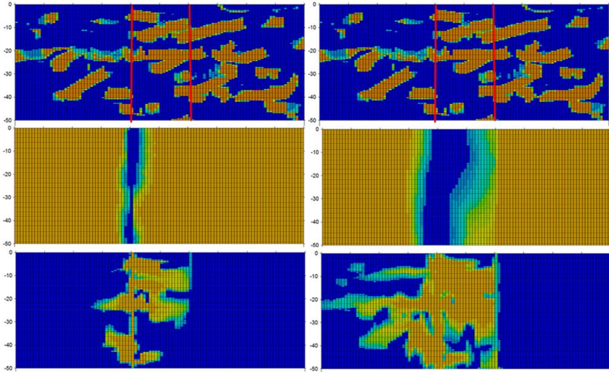
Figure 15: From top to bottom: horizontal permeability field and position of vertical wells (red lines), temperature and tracer fields after 1 year (left) and 10 years (right)
