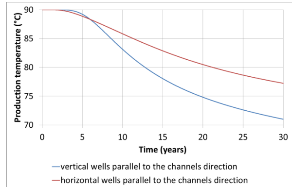
Figure 4: Evolution of the production temperature during exploitation for horizontal wells
