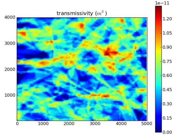
Figure 21: Productive layer transmissivity ( \text{m}^3 )
