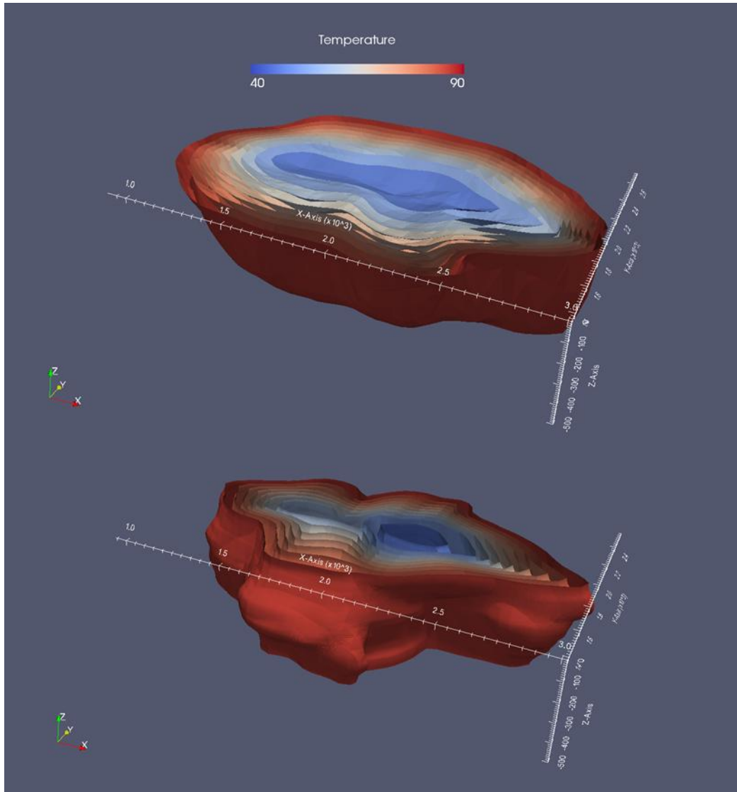
Figure 28: Comparison of the cold plume extension between the homogeneous model on the top and the heterogeneous model on the bottom. Case of horizontal wells.
