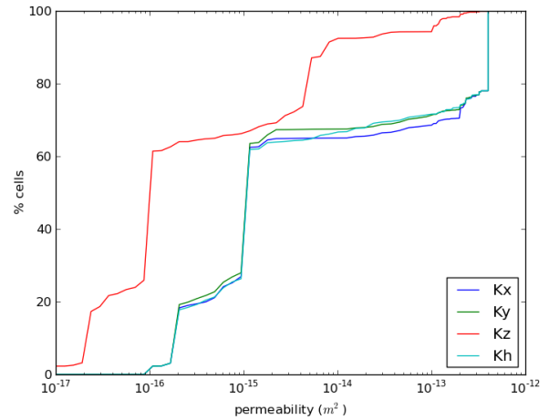
Figure 17: Distribution of permeability ( \text{m}^2 ) in the heterogeneous block
