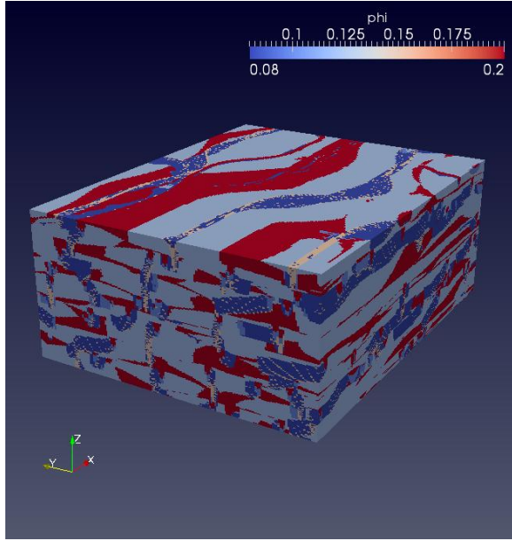
Figure2: Porosity values of the original block (6 million cells block with porosity values given by table 1) (40x vertical exaggeration)
