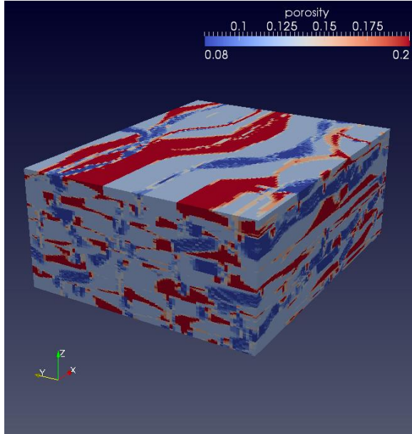
Figure3: Porosity values of the upscaled 800,000 cells block (40x vertical exaggeration)
