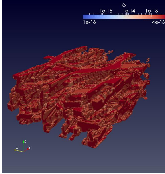
Figure 19: Cells of the coarse grid that have an horizontal permeability above the 5.10^{-14} \text{ m}^2 threshold ( K_h \geq K_{min} = 5.10^{-14} \text{ m}^2 ) (40x vertical exaggeration)
