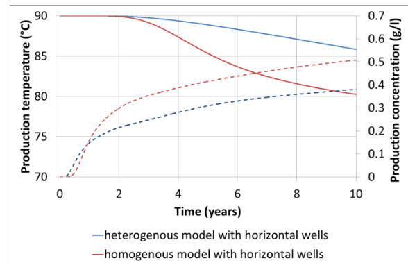
Figure 26: Comparison of the production temperature (solid lines) and tracer concentration (broken lines) between the heterogeneous model and the two-layer homogeneous model in the case of horizontal wells
