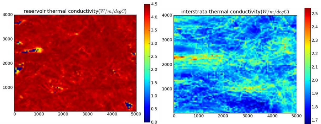
Figure 24: Reservoir and interstrata thermal conductivity (W/m/°C)
