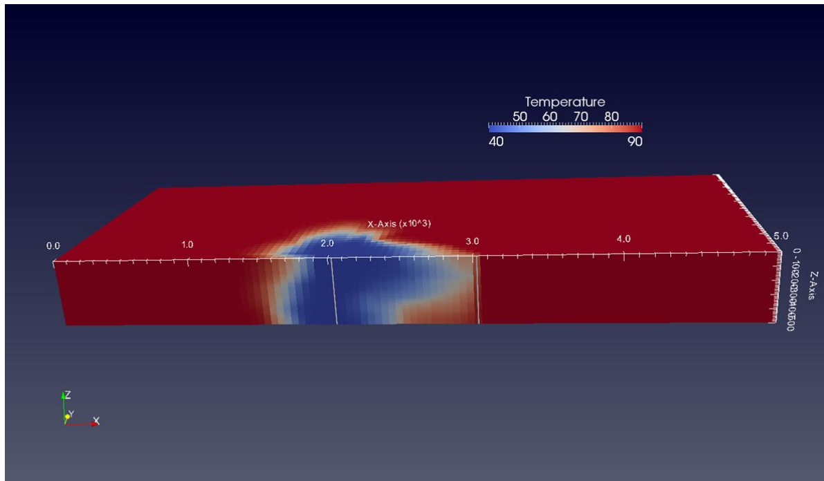
Figure 5: Cold plume extension after 10 years of geothermal exploitation (vertical wells positioned in parallel to channels, x direction).
