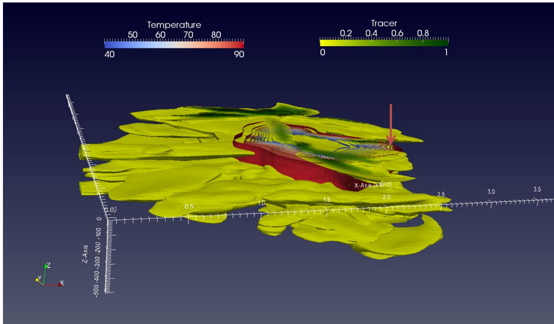
Figure 11: Temperature and tracer isocontours after 10 years of exploitation (vertical wells oriented according x direction).
