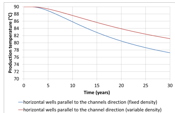
Figure 9: Comparison of the production temperature for horizontal wells between the simulation with and without density effect.
