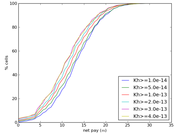
Figure 18: Distribution of the net pay (m) according to the permeability threshold
