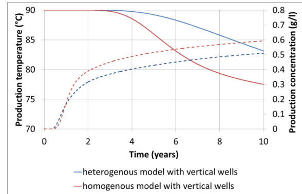
Figure 25: Comparison of the production temperature (solid lines) and tracer concentration (broken lines) between the heterogeneous model and the two-layer homogeneous model in the case of vertical wells
