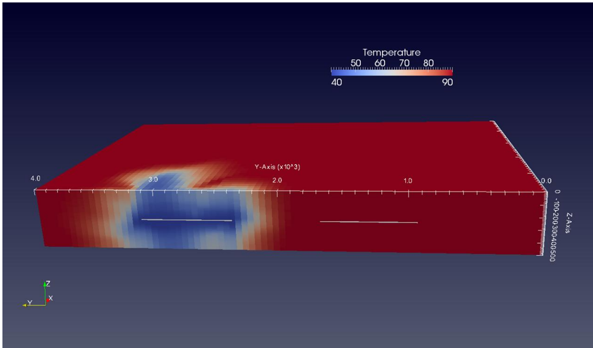
Figure 8: Cold plume extension after 10 years of geothermal exploitation (horizontal wells positioned perpendicularly to channels, y direction).
