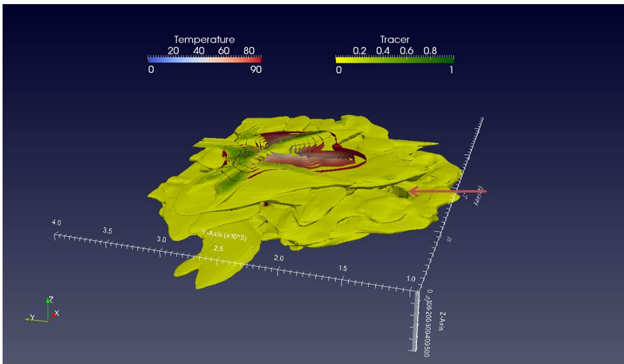
Figure 14: Temperature and tracer isocontours after 10 years of exploitation (horizontal wells oriented according y direction).
