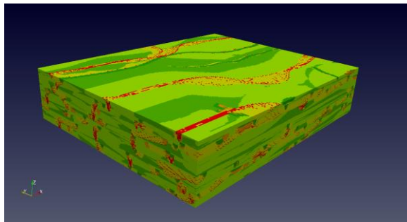
Figure 1: 3D lithofacies block from the Flumy model. (6 million cells) There are 9 different lithofacies (cf. table 1). Relatively permeable sandy facies are represented in red and yellow (channel lags, sand plugs, point bars) whereas more impervious facies are in shades of green (overbank deposits, alluvial plain) (20x vertical exaggeration)
