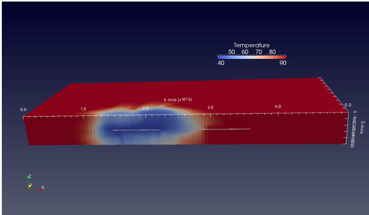
Figure 6: Cold plume extension after 10 years of geothermal exploitation (horizontal wells positioned in parallel to channels, x direction)
