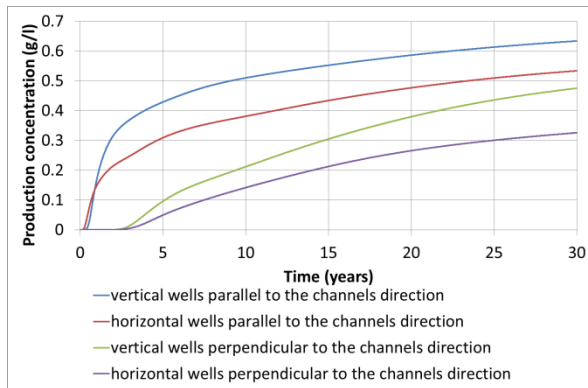
Figure 10: Production concentration curves
