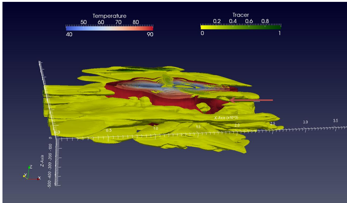
Figure 12: Temperature and tracer isocontours after 10 years of exploitation (horizontal wells oriented according x direction).
