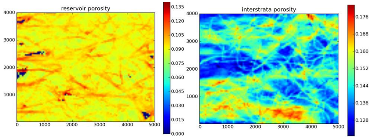
Figure 23: Reservoir and interstrata porosity
