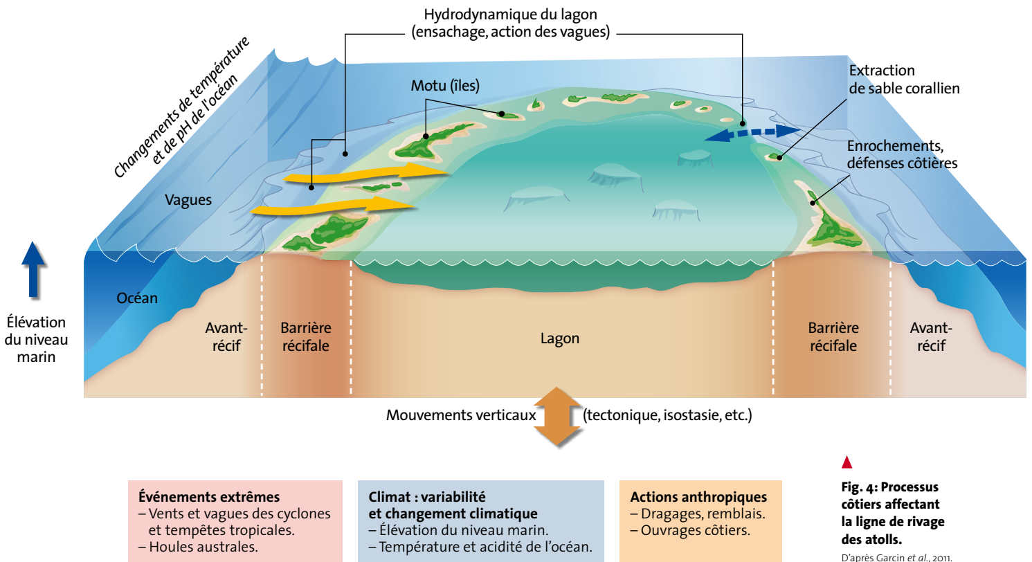
Fig. 4: Coastal processes affecting the shorelines of the atolls.
