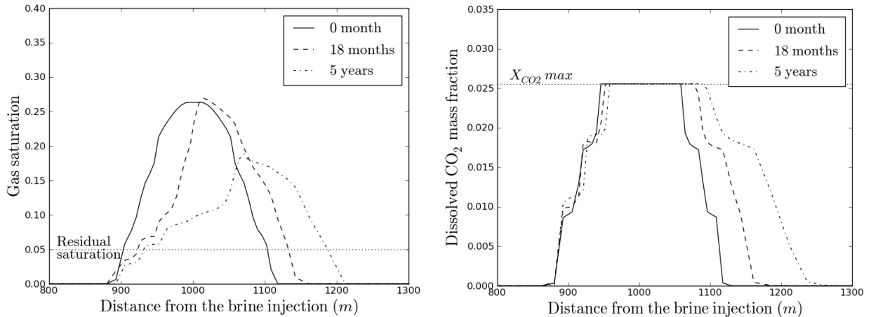
Figure 4: Gas saturation (left) and CO 2,aq mass fraction (right) in the upper aquifer (average of the three layers) in a vertical cross-section from the brine injection well (located at 0m) to the leak (located at 1000 m) after 0, 1.5 and 5 years of brine injection at 15 m 3 /h
