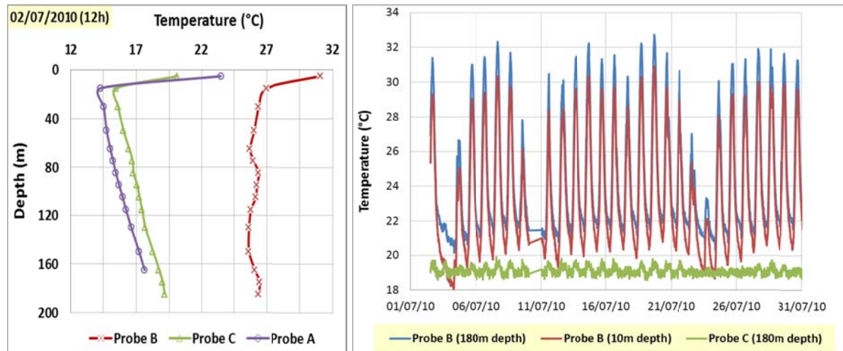
Figure 1: Temperature vertical distribution and temporal evolution in the schist rock after 3 months of solar thermal energy injection
