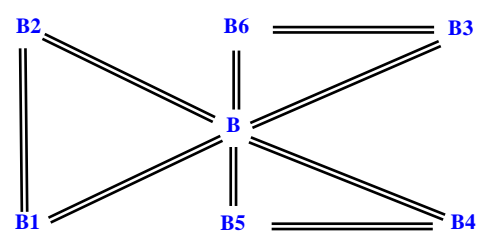
Figure 2.3.1.1 Horizontal \delta g grid measurement schedules at site B performed separately for heights of 30 cm, 90 cm and 130 cm
