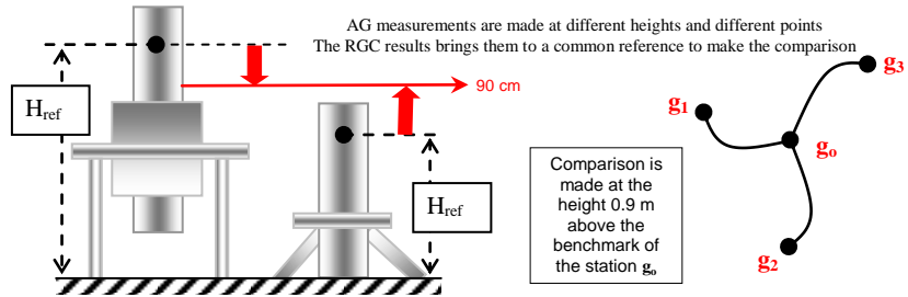
Figure 1.1 RGC2009 brings the absolute g -values measured at different stations ( g_0, g_1, g_2, g_3 ) at different heights to the same reference ( g_0 on 0.90 m above the ground benchmark) for comparison.
