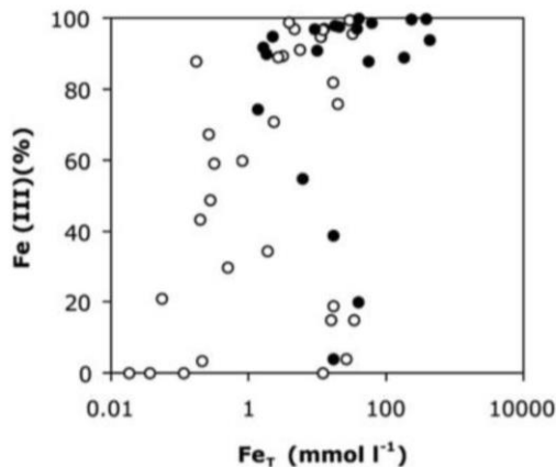
Fig. 3. Percentage of Fe(III) in solution as a function of total dissolved Fe (Fe T ). Samples analysed for Fe isotopes are in black.
