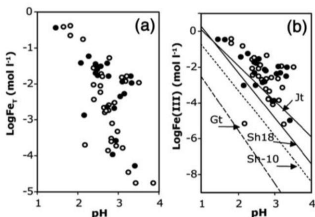
Fig. 2. Concentrations of total dissolved Fe (Fe T ) (a) and Fe(III) (b) versus pH. Samples analysed for Fe isotopes are in black. Theoretical solubility lines for schwertmannite (Sh), goethite (Gt) and jarosite (Jt) are also represented. The following reactions and constants are used: Schwertmannite (Sh-10): Fe 8 O 8 (OH) 4.4 (SO 4 ) 1.8 + 20.4 H + = 8 Fe 3+ + 1.8 SO 4 2- + 12.4 H 2 O; LogKs = 10.5, Yu et al. (1999). Schwertmannite (Sh-18): Fe 8 O 8 (OH) 4.8 (SO 4 ) 1.6 + 20.8 H + = 8 Fe 3+ + 1.6 SO 4 2- + 12.8 H 2 O; LogKs = 18, Bigham et al. (1996). Goethite (Gt): FeOOH + 3 H + = Fe 3+ + 2 H 2 O; LogKs = 0.5, Parkhurst and Appelo (1999). Jarosite (Jt): KFe 3 (SO 4 ) 2 (OH) 6 + 6 H + = K + + 3 Fe 3+ + 2 SO 4 2- + 6 H 2 O; -14.8, Parkhurst and Appelo (1999). *Calculation have been made for Log(SO 4 2- ) = -2.74, which represents a bottom limit for SO 4 2- activity in AMD (higher SO 4 2- activities would shift down the solubility lines).
