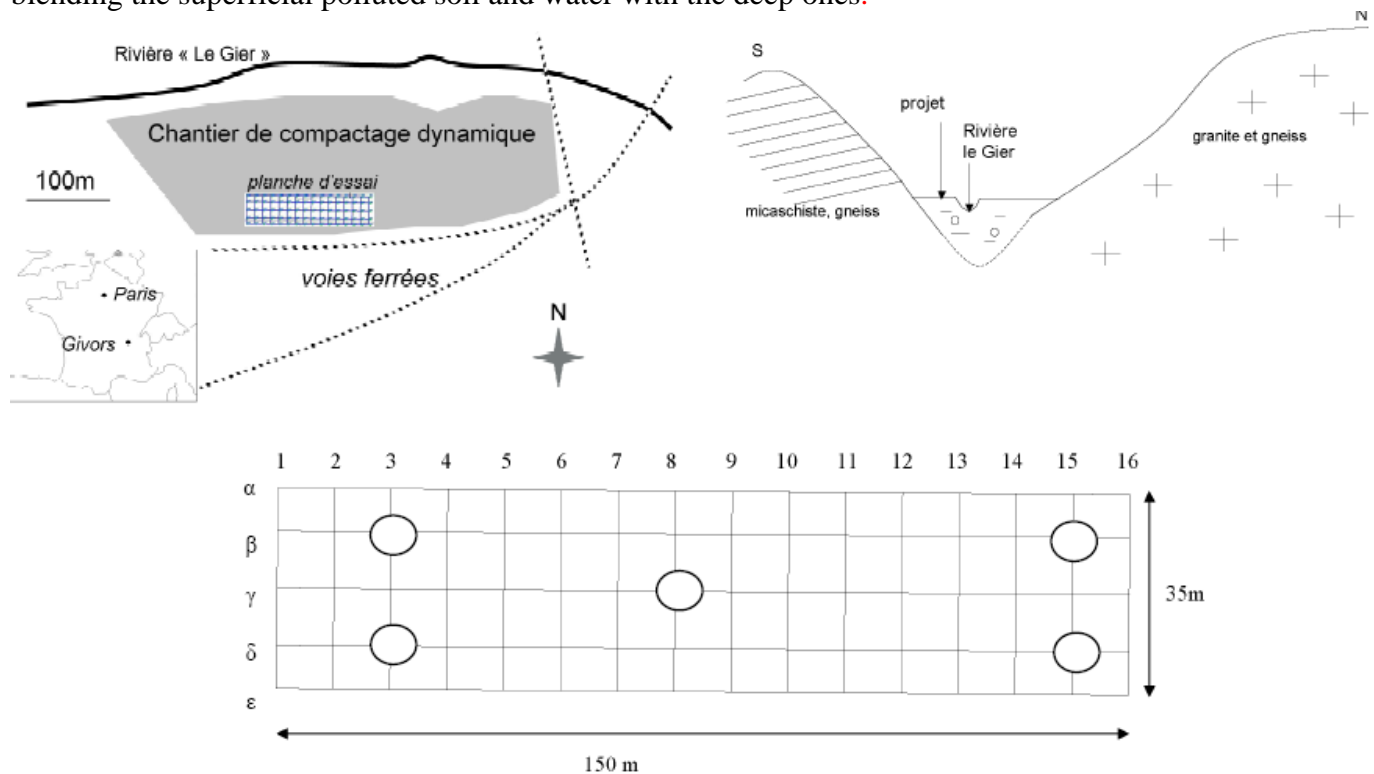
Fig.1: Location map of project (top left) and schematic geological cross-section (top right) Bottom, location and plan view of the test board. The five circles indicate the position of the static penetrometers
