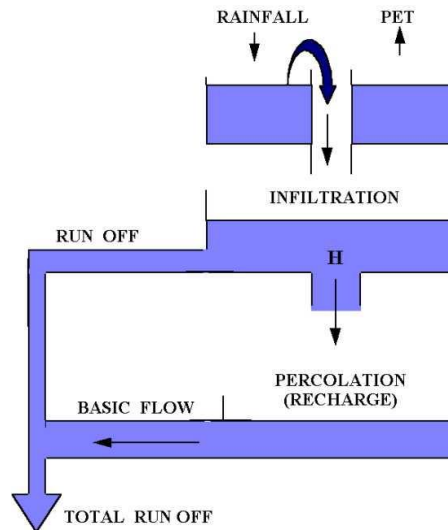
Figure 1: Schematic representation of GARDÉNIA®'s operating principle
