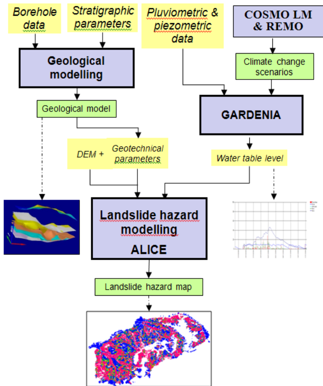
Figure 2: Chain of the methodology for coupling the hazard assessment tool with the hydrological model
