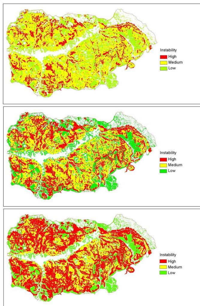
Figure 5: Representation of instability resulting from the simulations using the 3 different filling ratios. The ratio is 0 (top), 0.5 (middle) and 1 (bottom).
