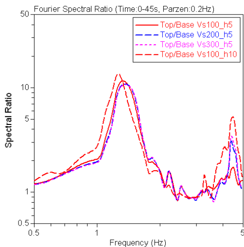
Figure 7. Spectral Ratios computed between top and base of the 0.5s model for three soil conditions ( V_s=100, 200 and 300 m/s) and two soil thicknesses ( h=5 m and 10 m)
