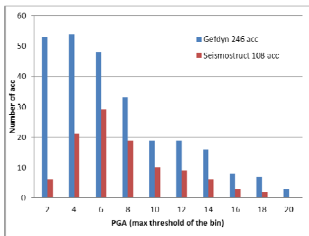
Figure 5. Histogram of the PGA ( \text{m/s}^2 ) values for the time-histories used for dynamic analyses
