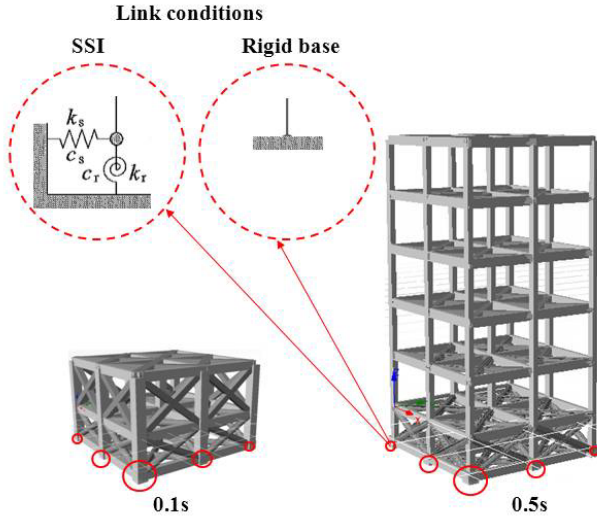
Figure 3. Models for non-linear time history analysis (two-step approach)
