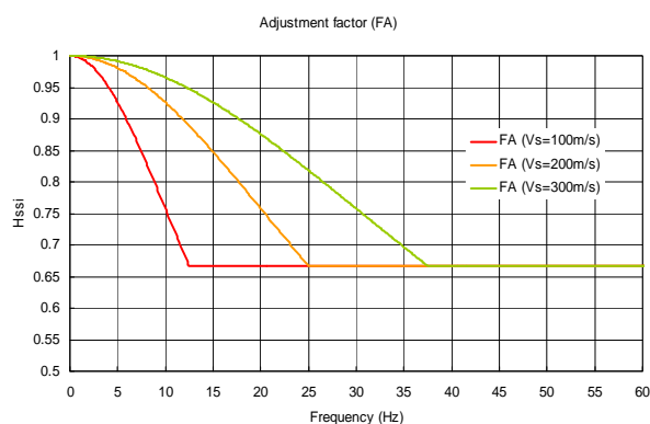
Figure 4. Adjustment factor (FA) of the embedded foundation for three soil conditions: V_s=100, 200 and 300\text{m/s}
