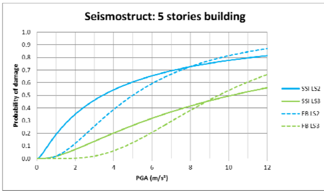
Figure 9. Fragility curves for 5 story buildings developed using two-step approach
