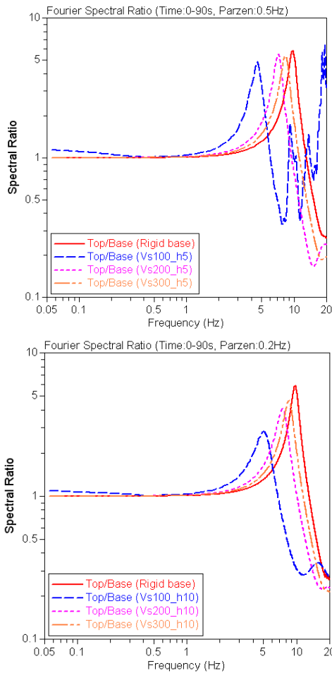
Figure 6. Spectral Ratios computed between top and base of the 0.1s model for three soil conditions ( V_s=100, 200 and 300 m/s) and two soil thicknesses ( h=5 m and 10 m)
