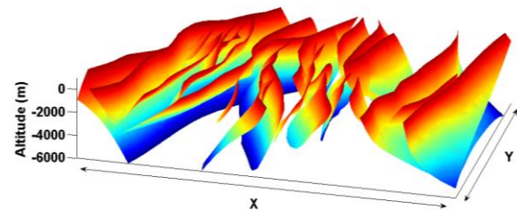
Figure 4: 3D representation of the fault planes
