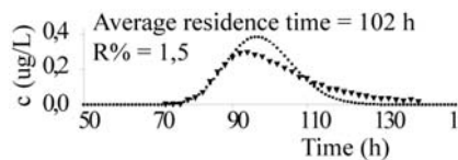
Figure 3 :Artificial tracer test recovery curve at the Loiret spring realized in October 2009 (triangle) and best fit from 1D solution with x=13\text{km} ; D=55\text{ m} ; A_{nr}=10\text{m}^2 ; \Delta M=1\text{kg} ; u=3,6\text{ cm/s} ; \lambda=1,25\cdot 10^{-5}\text{ s}^{-1} (square). .
