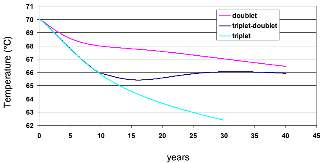
Figure 13: Production well temperature for the three types of rehabilitation
