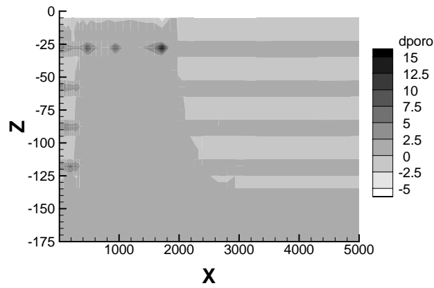
Fig. 23. Porosity changes after 10 000 years of simulation. dporo = 100 \times (\phi - \phi_{init}) / \phi_{init} . A porosity increase ( dporo > 0 ) of up to 15 % occurs in the shales, while a slight decrease ( dporo < 0 ) of less than 5 % is seen in the sands.
