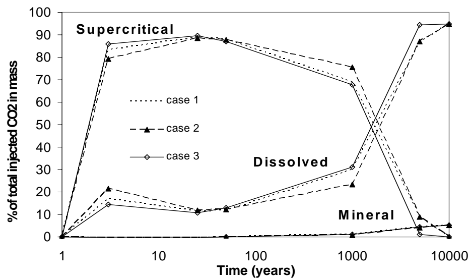
Fig. 26. Comparison of \text{CO}_2 inventories in the different phases for three different cases: Case 1 with the original mesh and a residual saturation of 0.20, Case 2 with the same mesh and a reduced residual gas saturation of 0.05, and Case 3 with a residual gas saturation of 0.20 and a mesh that is more refined near the injection point.
