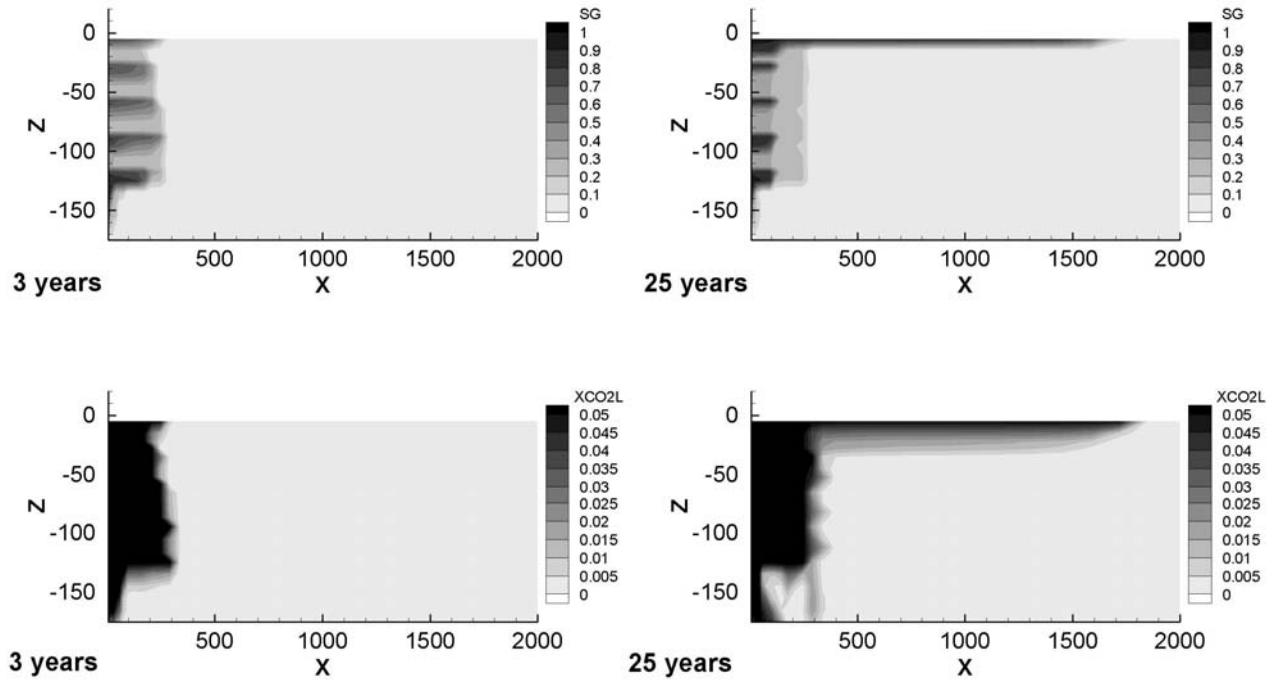
Fig. 7. Gas saturations (SG) and mass fractions of dissolved CO 2 in the liquid phase (XCO 2 L), after 3 years of injection and at the end of the injection period (25 years).
