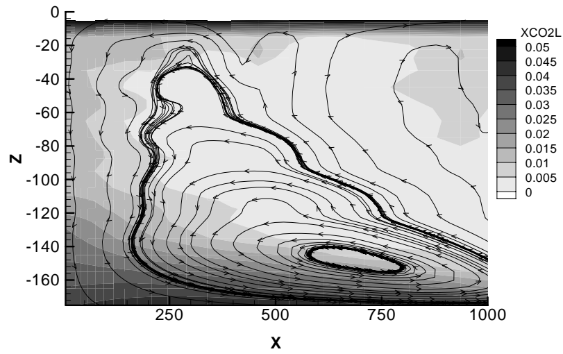
Fig. 10. Streamlines and dissolved \text{CO}_2 mass fractions X_{\text{CO2L}} in the brine after 2,000 years. The streamlines highlight the convective fluid circulation induced by the mixing of brines containing dissolved \text{CO}_2 .
