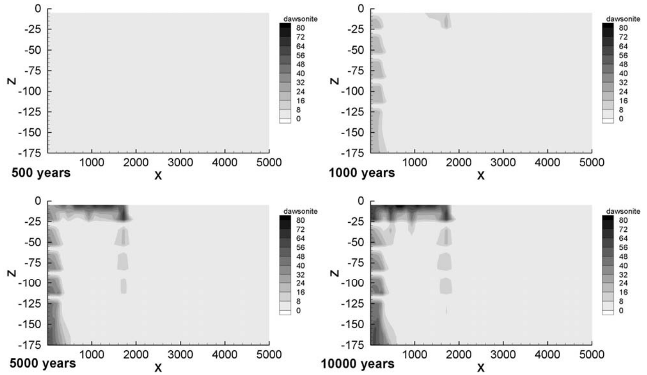
Fig. 16. Dawsonite mineral evolution in moles per \text{m}^3 of rock medium (negative sign for dissolution, positive sign for precipitation) after 500, 1000, 5000 and 10 000 years, following 25 years of injection of supercritical \text{CO}_2 .
