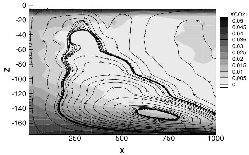
Fig. 10. Streamlines and dissolved CO 2 mass fractions XCO2L in the brine after 2,000 years. The streamlines highlight the convective fluid circulation induced by the mixing of brines containing dissolved CO 2 .
